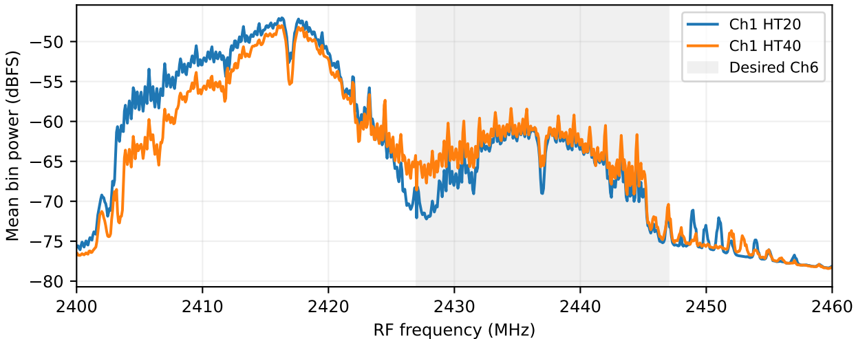
Ch1 bandwidth comparison; LO=2427 MHz, gain 20
