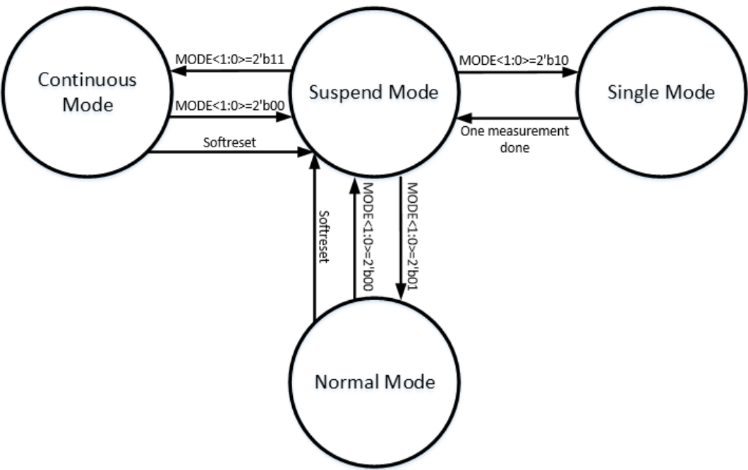
Figure 9. Modes Transition
