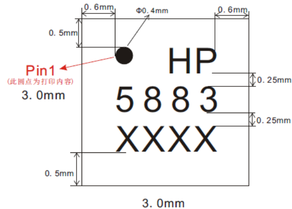
Figure 5. Chip Marking
