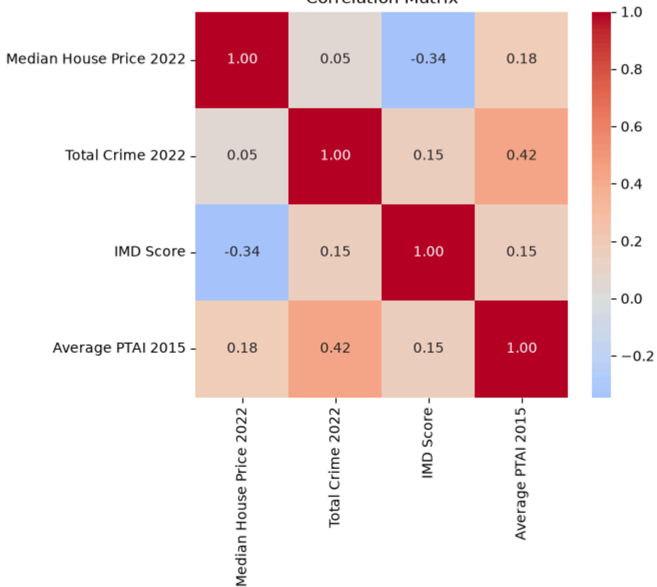
Correlation Matrix
