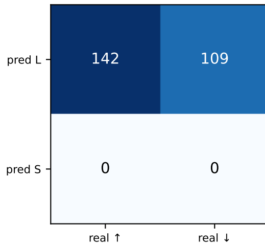
ZeroR acc = 0,57
