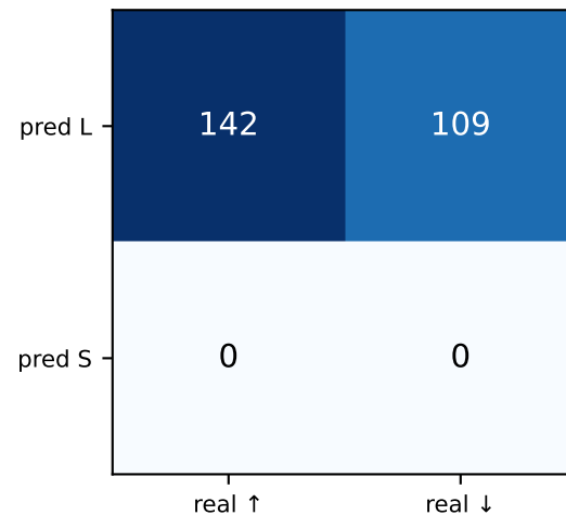
B&H acc = 0,57
