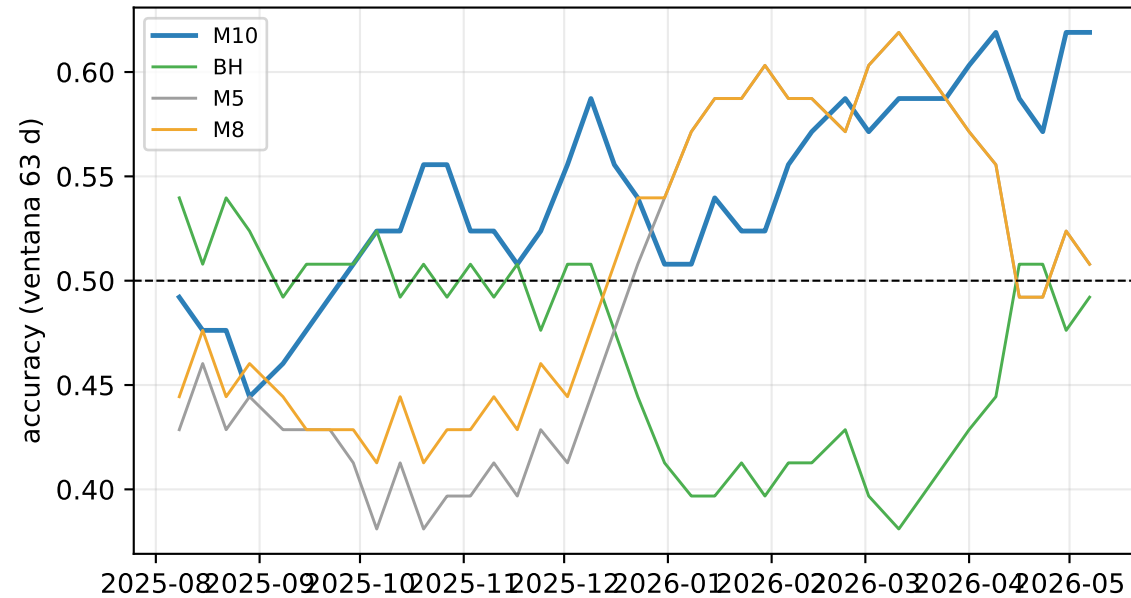
Accuracy rodante
