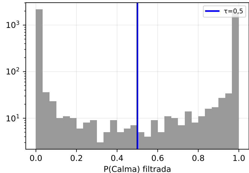
RAM score bimodal
