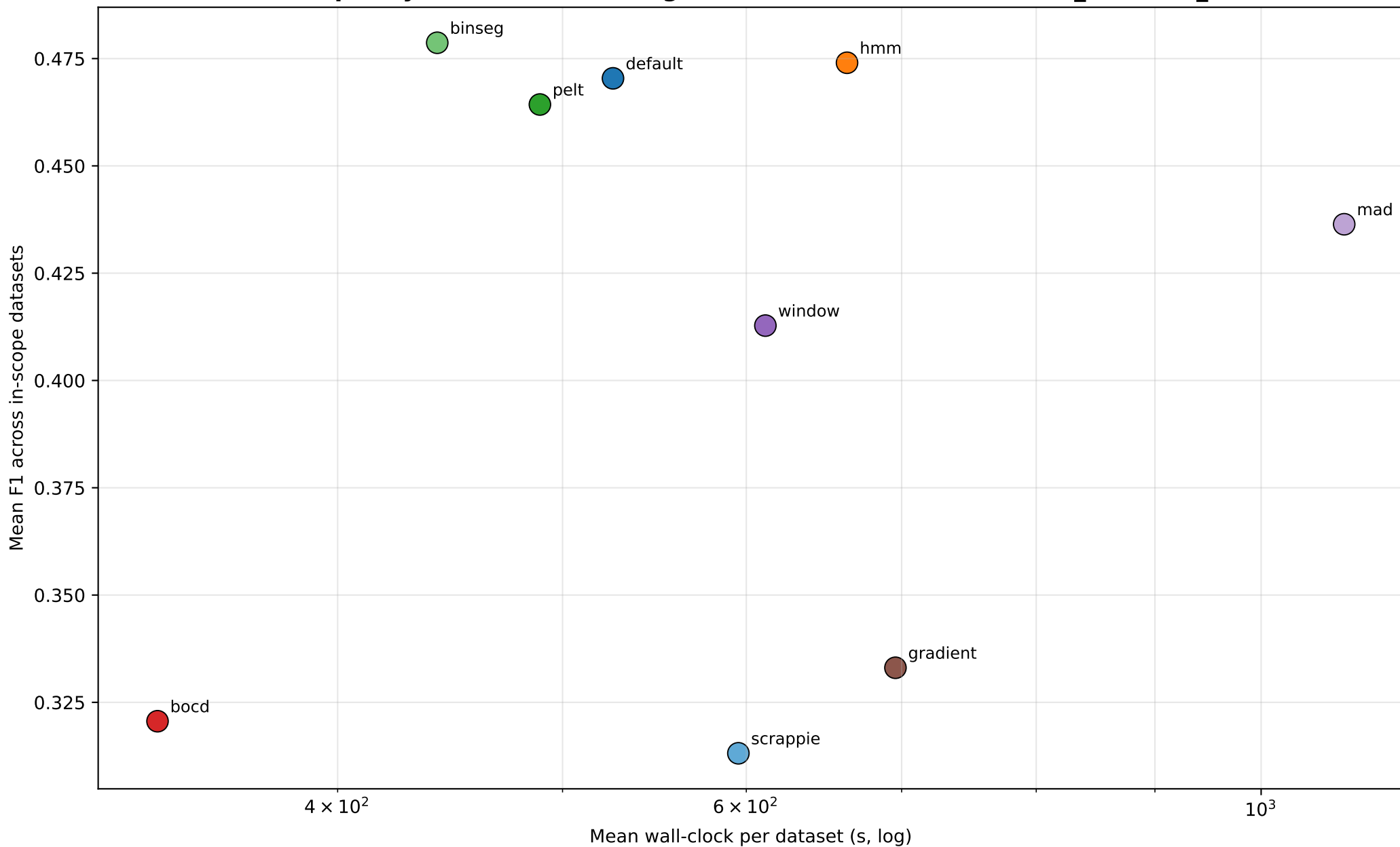
Pareto: quality vs runtime (averaged across D1,D2,D3,D4,D6, RB_dmel, RB_ecoli)
