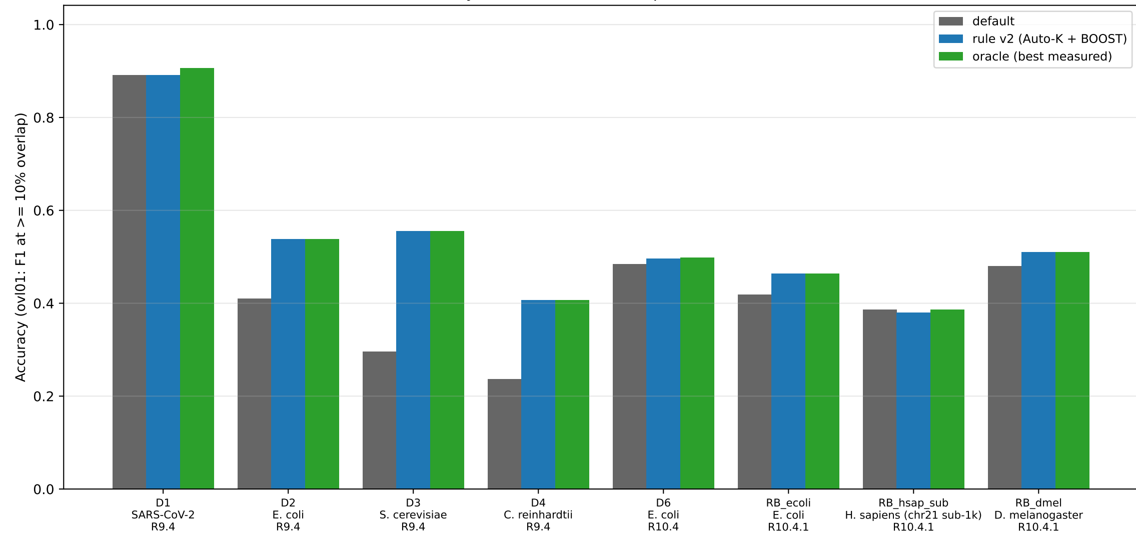
Accuracy: default vs rule v2 vs per-dataset oracle
