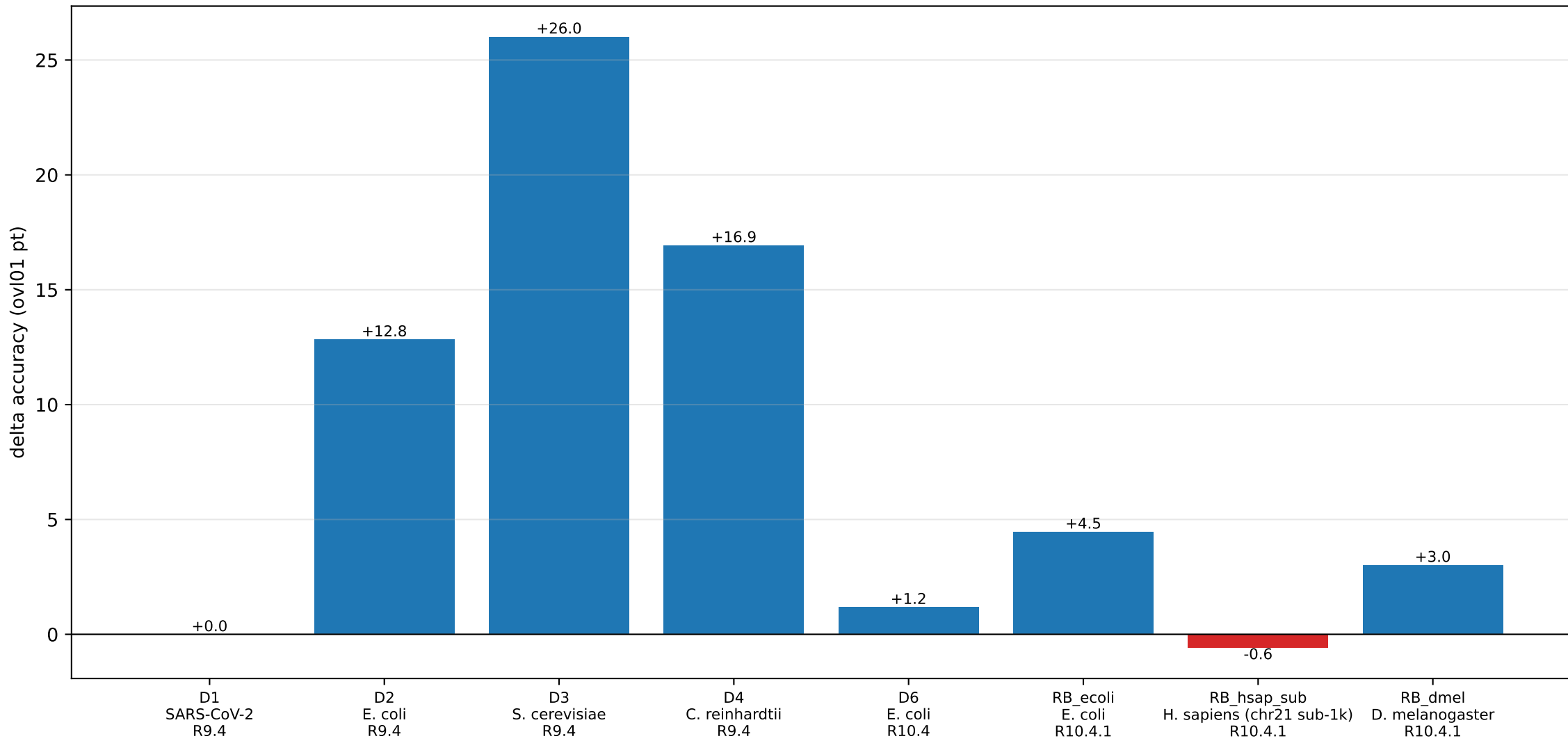
Accuracy delta: rule v2 - default (positive = better)
