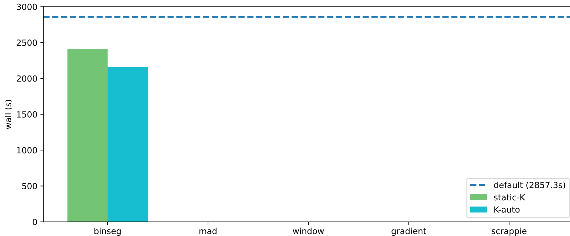
D6 — wall time (sequential, exclusive node) vs default = 2857.3s
