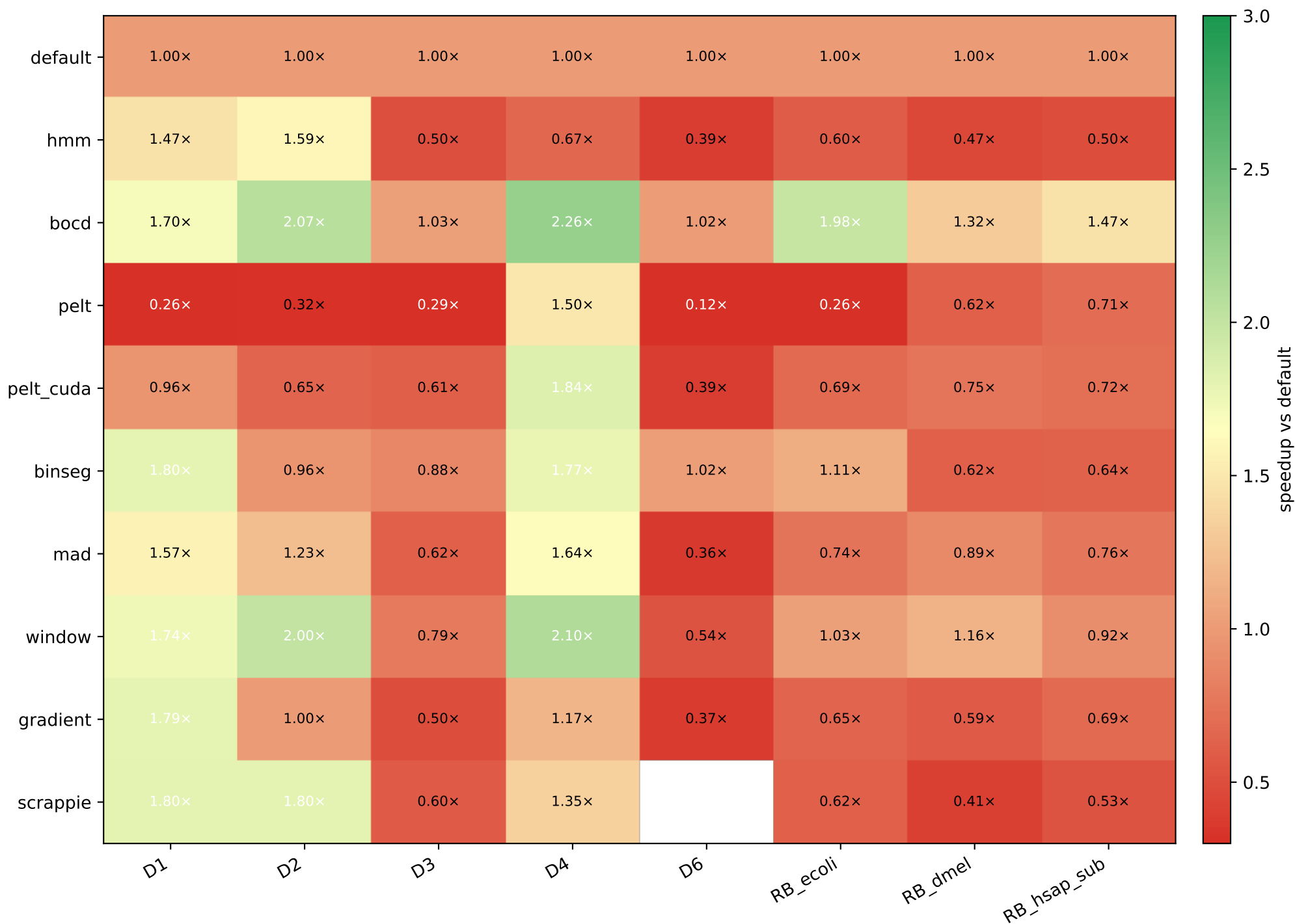
Wall-time speedup vs default — best mode per segmenter
