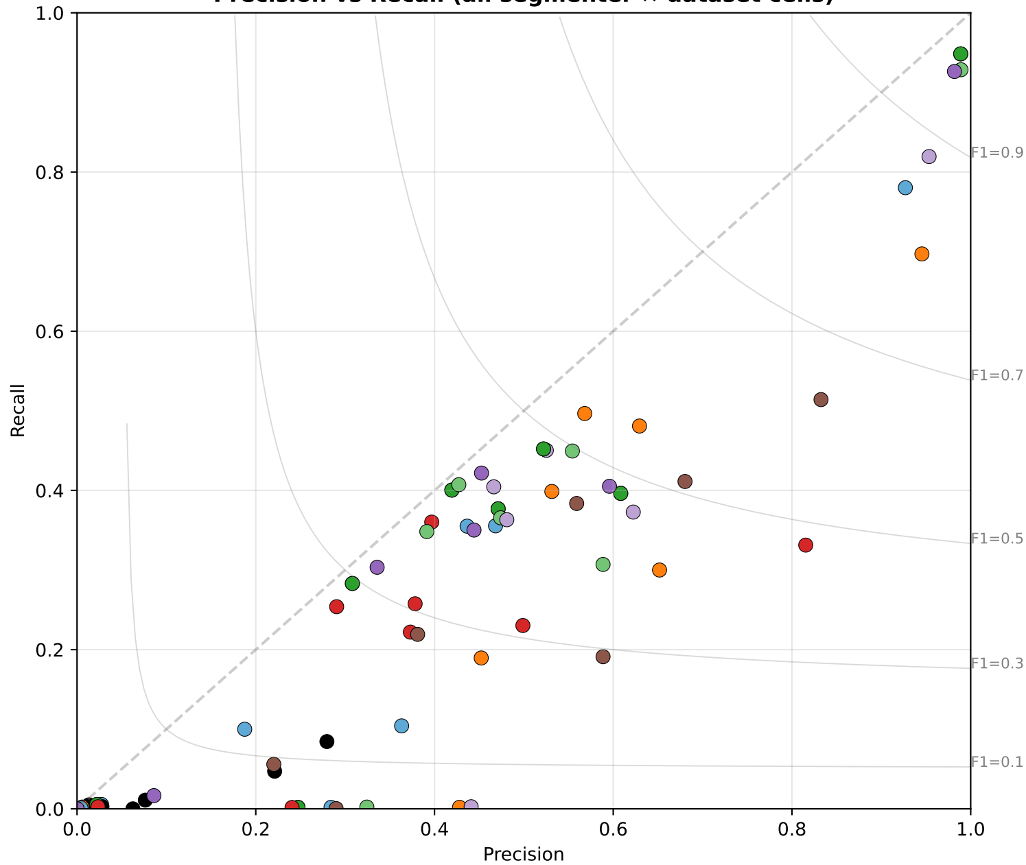
Precision vs Recall (all segmenter x dataset cells)
