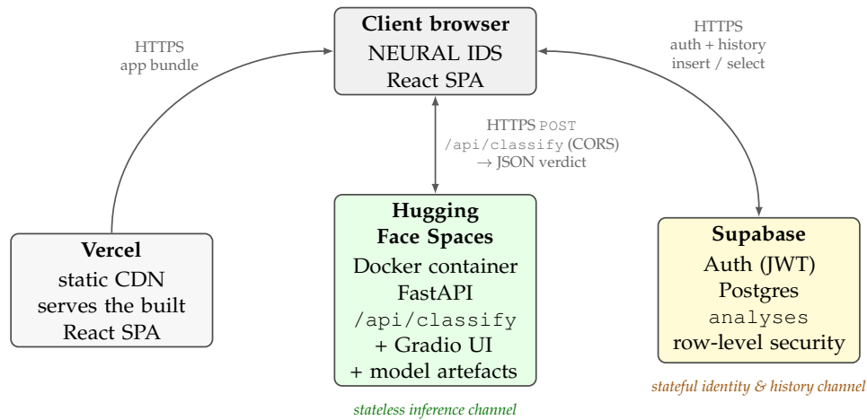
Figure 4.1: Runtime deployment topology of the serving subsystem. Vercel delivers the static React SPA (grey); at runtime the SPA drives two independent backends: a stateless inference service on Hugging Face Spaces (green) reached via POST /api/classify , and a stateful Supabase project (yellow) for authentication and per-user history. The two channels share no server-side state, so inference never blocks on persistence and either tier can be replaced in isolation.
