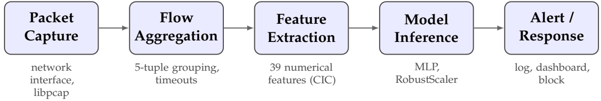
Figure 2.1: End-to-end architecture of a real-time deep learning-based intrusion detection system.
