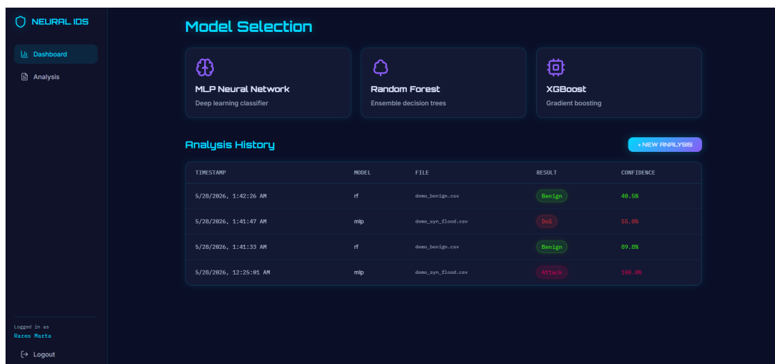
Figure 4.1: NEURAL IDS dashboard after the F1 acceptance runs. The analysis history table records four classification requests: the SYN-flood capture classified as Attack (near-certain binary confidence) and as DoS ( \approx 55\% ) under different granularities, and the benign capture classified as Benign. The three model-selection cards at the top set the model_type field of subsequent API calls. (Screenshot is illustrative; binary confidence is reported after temperature scaling in the text.)
