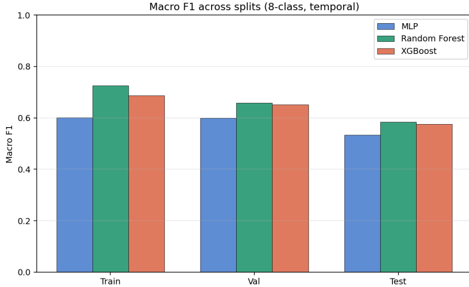
Figure 5.11: Macro F1 across train / validation / test partitions (8-class granularity). Macro F1 (which weights all classes equally regardless of frequency) is substantially lower than Weighted F1 for all models, revealing that minority-class detection remains challenging. All three models decline monotonically from train to test, and the MLP’s macro F1 ( \approx 0.53 on test) trails the tree ensembles ( \approx 0.58 ), confirming that the deep model’s disadvantage is concentrated in the rare attack families.
