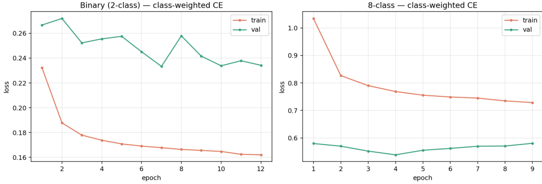
Figure 5.7: MLP training and validation loss (class-weighted cross-entropy) on the temporal split. Left: binary (2-class) granularity, reaching its best validation loss around epoch 7 and early-stopping at epoch 12. Right: 8-class granularity, best around epoch 4 and early-stopping at epoch 9. In both cases early stopping triggers at patience=5 after the best validation checkpoint is reached. Note that in the 8-class case the validation loss is consistently lower than the training loss: this inversion is expected under class-weighted cross-entropy when the minority-class weights impose a steeper penalty on training-set errors than on the validation set.
