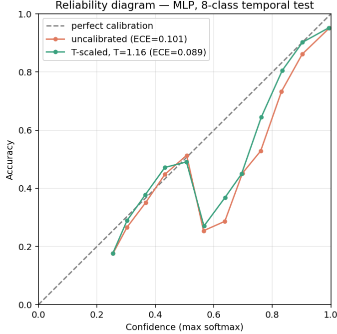
Figure 5.14: Reliability diagram for the MLP on the temporal-split 8-class test set, before and after temperature scaling. Points below the diagonal indicate overconfidence. Temperature scaling ( T = 1.16 , fitted on the validation set) pulls the curve towards the diagonal, reducing ECE from 0.101 to 0.089.
