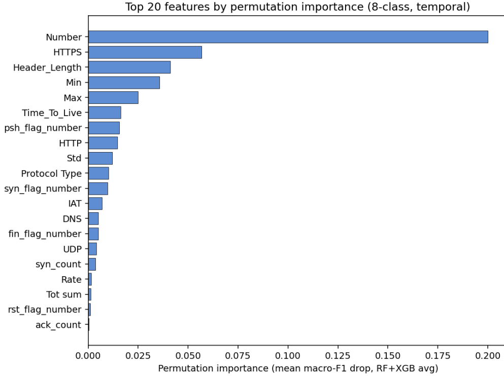
Figure 5.6: Top 20 features by average permutation importance (drop in macro-F1 under feature shuffling) across the Random Forest and XGBoost baselines (8-class, temporal split). The packet-count feature Number dominates by a wide margin, followed by the HTTPS protocol indicator, Header_Length , and the packet-length statistics Min and Max . The long low-importance tail confirms that the pruned 25-feature set carries little redundant signal.
