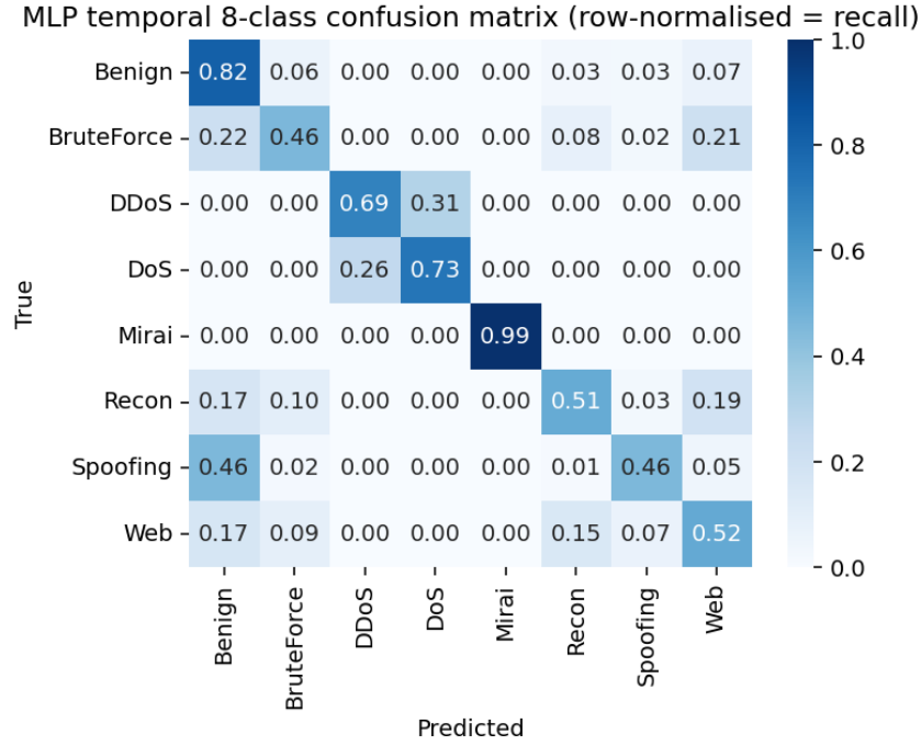
Figure 5.9: Row-normalised confusion matrix (per-class recall) for the MLP on the temporal-split 8-class test set. Rows represent true labels; columns represent predicted labels. Diagonal values are per-class recall. The Mirai family achieves near-perfect detection (0.99); DDoS and DoS are frequently confused with each other; Spoofing and Recon bleed substantially into Benign.
