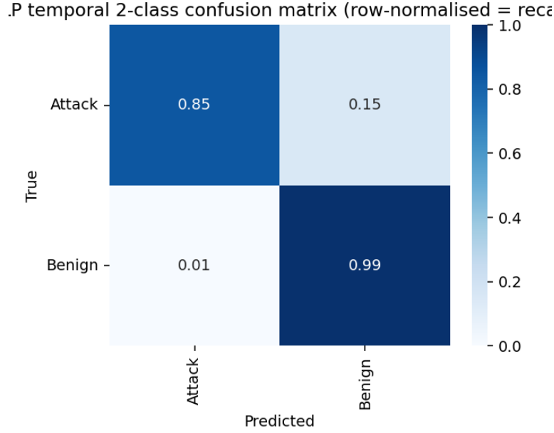
Figure 5.8: Row-normalised confusion matrix (per-class recall) for the MLP on the temporal-split 2-class test set. Diagonal values are recall: Attack recall = 0.85, Benign recall = 0.99.
