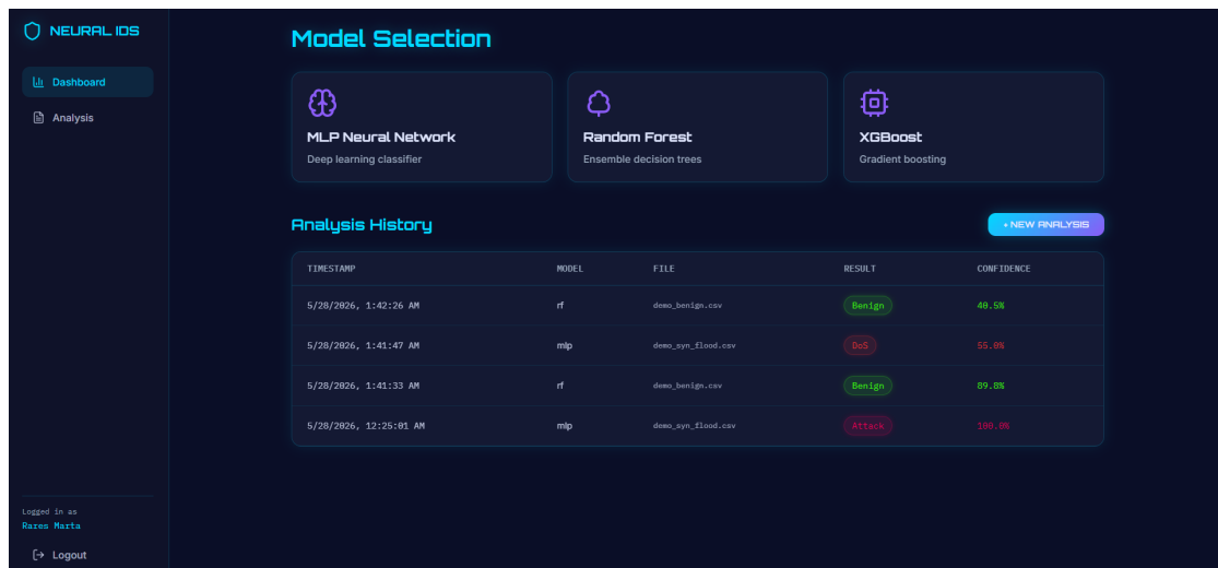
Figure 4.2: NEURAL IDS dashboard after the F1 acceptance runs. The analysis history table records four classification requests: the SYN-flood capture classified as Attack (near-certain binary confidence) and as DoS ( \approx 55\% ) under different granularities, and the benign capture classified as Benign. The three model-selection cards at the top set the model_type field of subsequent API calls. (Screenshot is illustrative; binary confidence is reported after temperature scaling in the text.)
