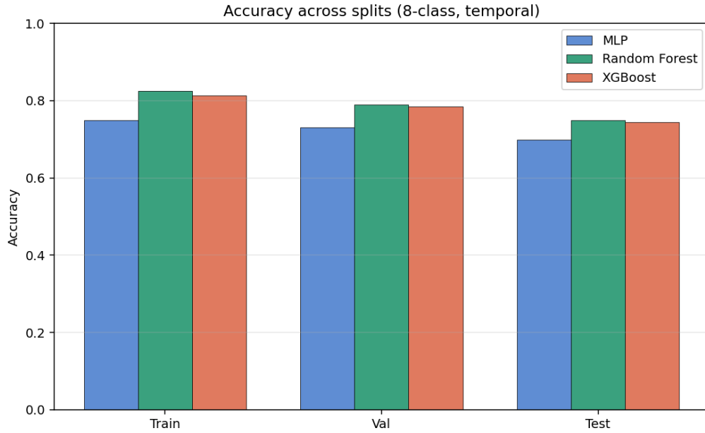
Figure 5.12: Accuracy at train, validation, and test partitions (8-class granularity). The MLP (0.698 test accuracy) lags the tree ensembles (RF: 0.750, XGBoost: 0.745) by roughly 5 percentage points. All models generalise stably, with a test-to-train accuracy drop below 8 percentage points.
