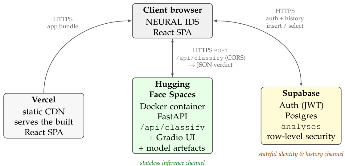
Figure 4.1: Runtime deployment topology of the serving subsystem. Vercel delivers the static React SPA (grey); at runtime the SPA drives two independent backends — a stateless inference service on Hugging Face Spaces (green) reached via POST /api/classify , and a stateful Supabase project (yellow) for authentication and per-user history. The two channels share no server-side state, so inference never blocks on persistence and either tier can be replaced in isolation.
