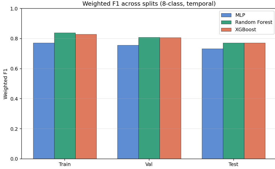
Figure 5.10: Weighted F1 across train / validation / test partitions for the three models on the temporal split (8-class granularity). All three models exhibit stable degradation from train to test. The tree ensembles (RF, XGBoost) achieve higher test weighted F1 ( \approx 0.771 ) than the MLP ( \approx 0.733 ), a gap of roughly 4 percentage points.
