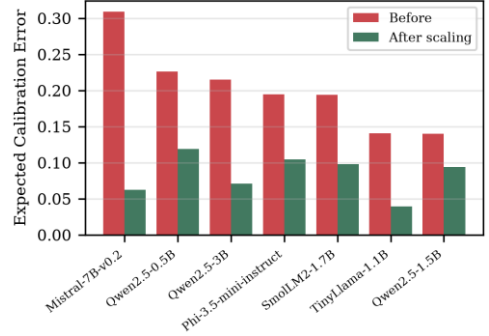
Fig. 2. Expected Calibration Error before and after temperature scaling for the seven models calibrated in this study. Every model is overconfident before correction; the 4-bit large model requires the largest temperature.
