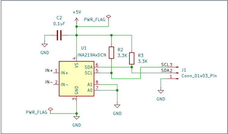
INA219 BLOCK
