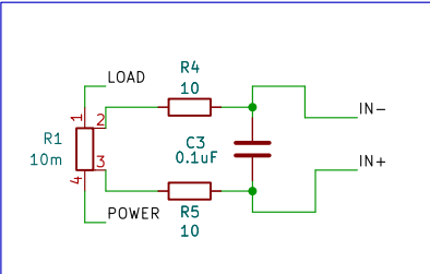
SHUNT RESISTOR KEVIN CONNECTION BLOCK
