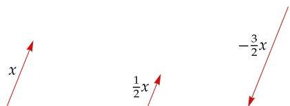
Scalar multiplication.
