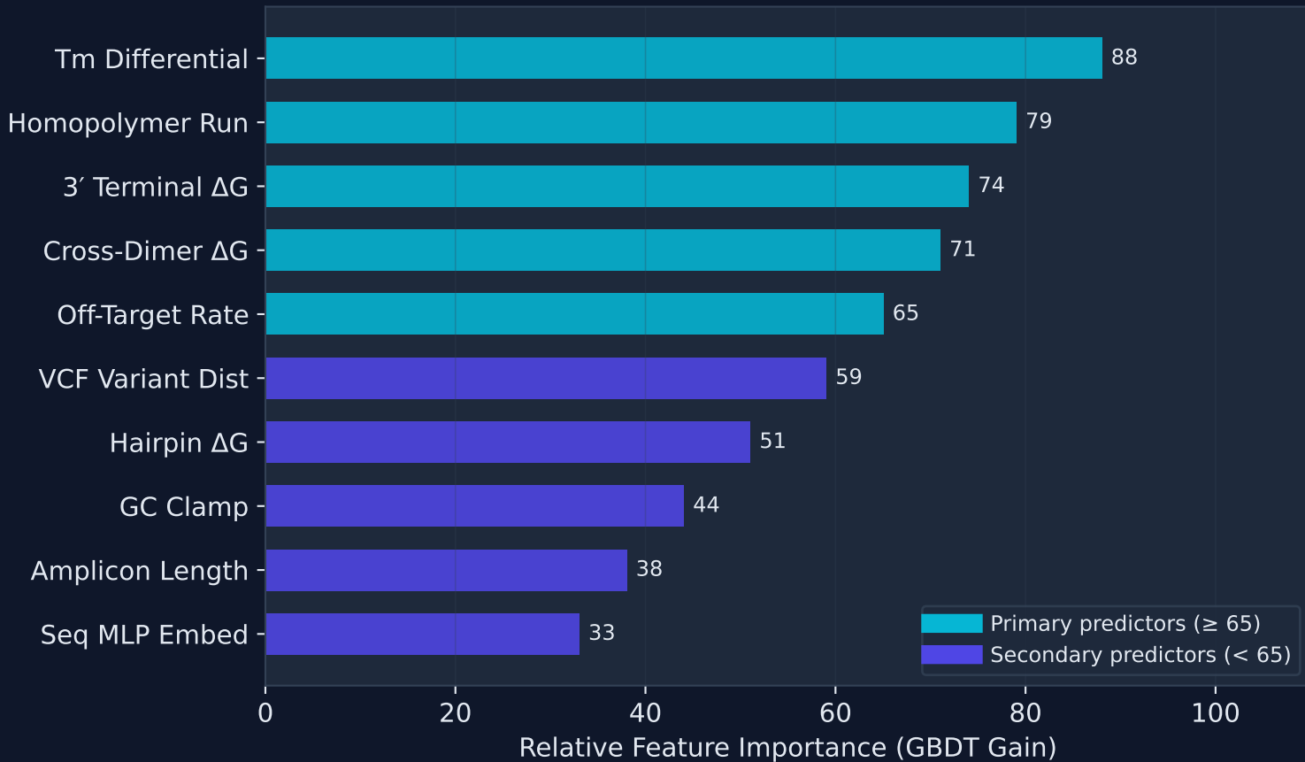
Figure 3 — PrimerForge Feature Importance (Stacked GBDT×5 Ensemble)
