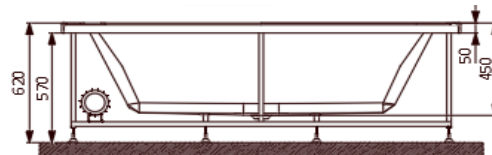
Bathtub with MS Frame
