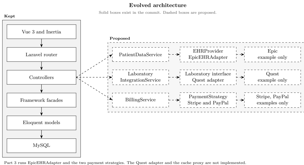
Figure 2. Evolved architecture. The left band is the application we inspected. The dashed band is proposed.
