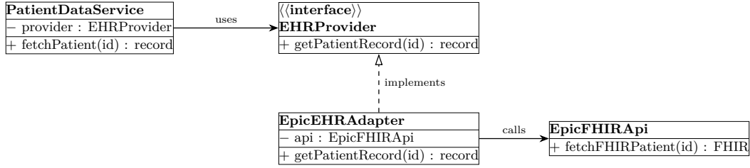
Figure 3. Adapter class diagram for the proposed EHR integration.
