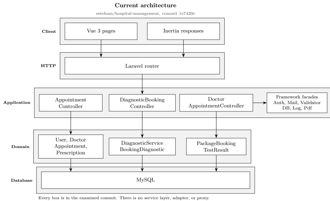
Figure 1. Current architecture. The shaded bands are the layers that exist today.
