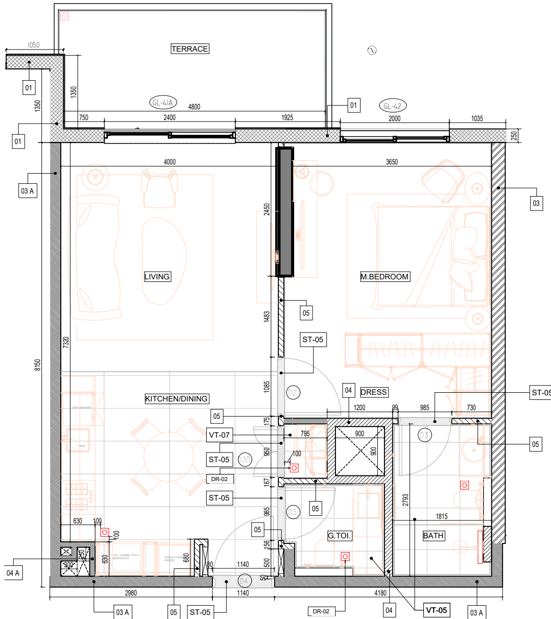
1 HILL 01 - LEVEL 1 - 1B A1-MASTER PLAN 1:25
