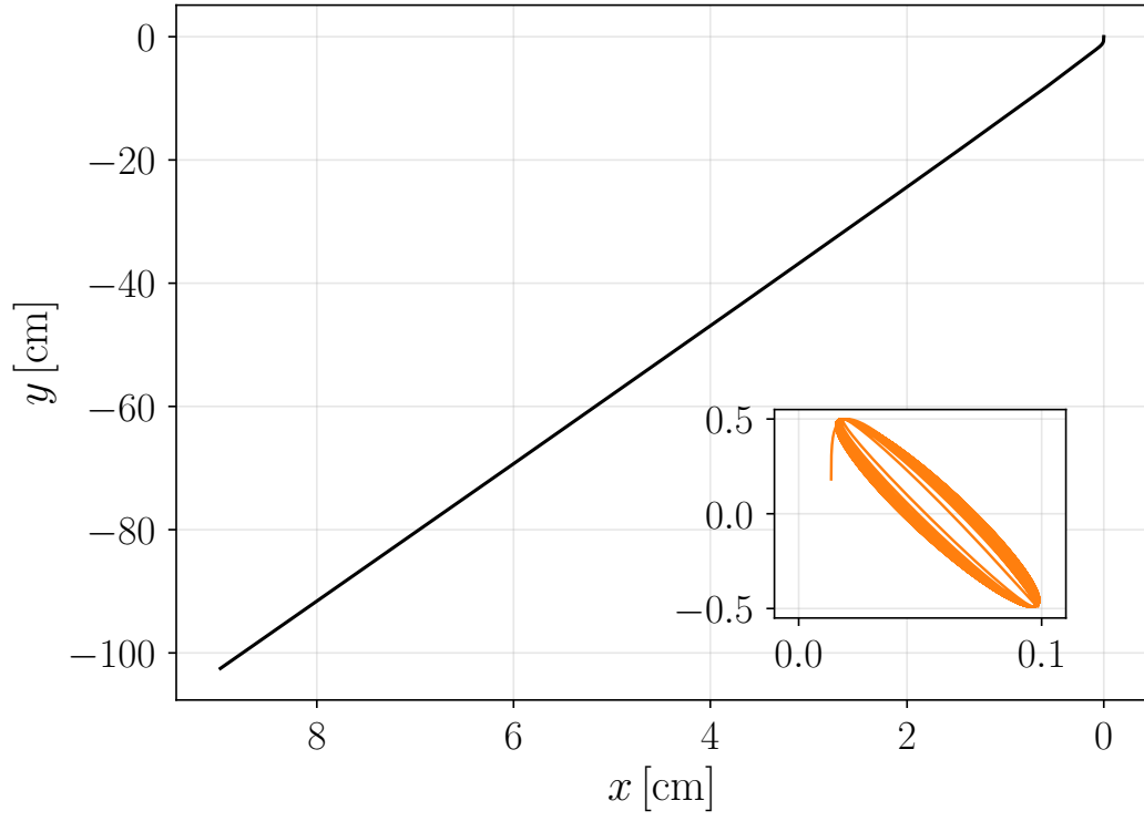
Figure K1: Shown is is the trajectory in the xy -plane and the evolution of the magnetic moment vector's direction (i.e. a point on the sphere in the direction of \boldsymbol{\mu} ).
