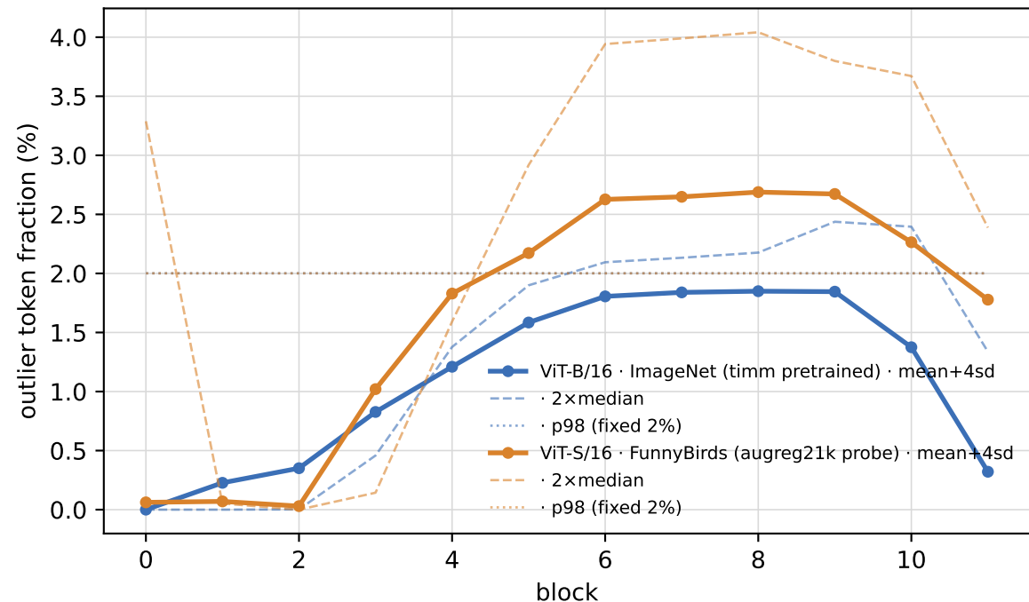
Outlier fraction per block — plateau \approx 2\text{--}3\% from block \sim 5\text{--}6 (criterion-insensitive)
