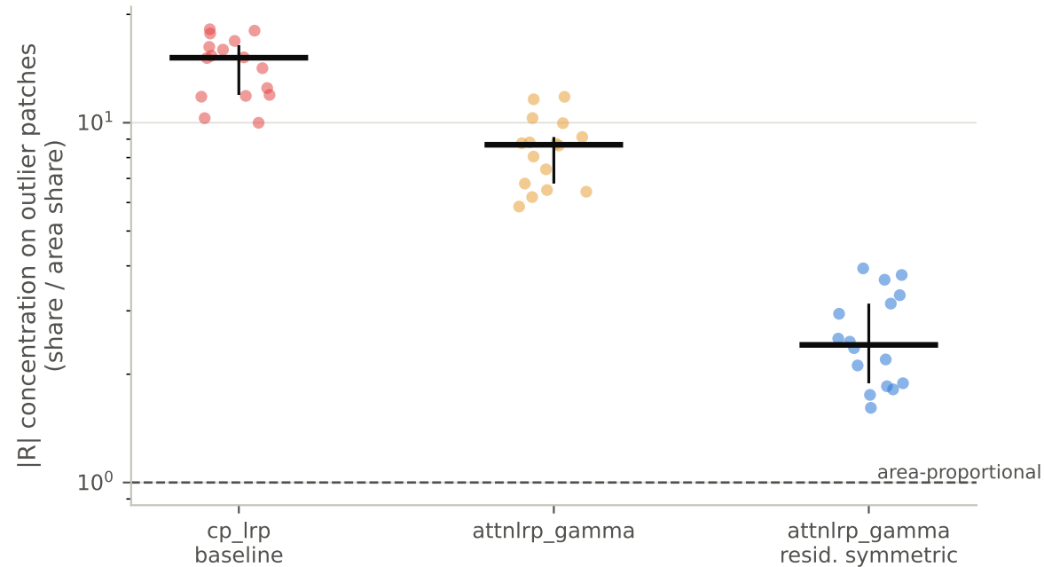
input-relevance mass on register patches, M=16 images
