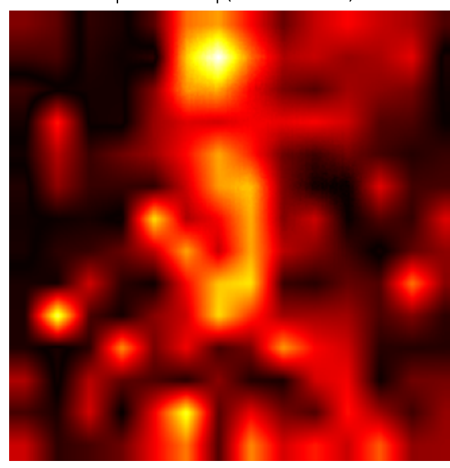
|d-mask224| (max=6.1e-06)
