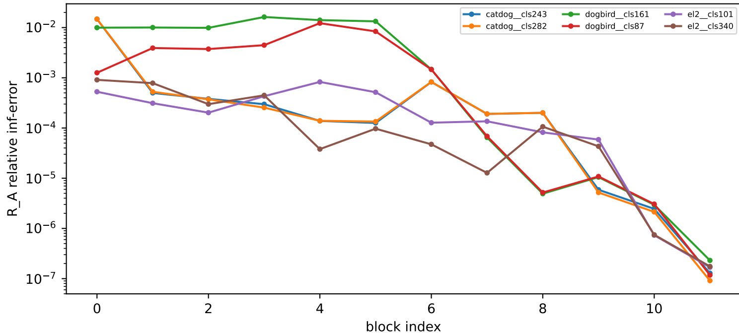
Per-block R_A error (decreases toward seed at block 11)
