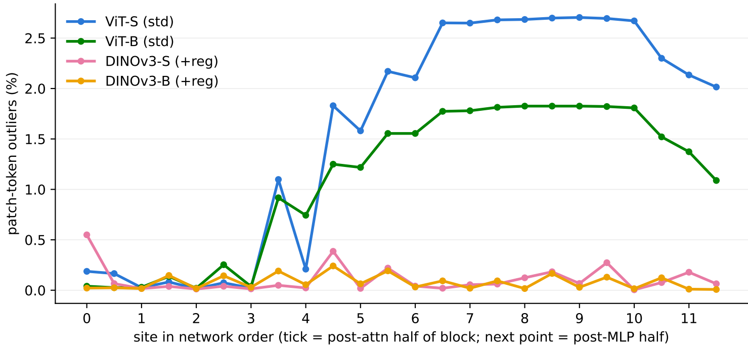
E1 — outlier fraction per half-block site (per-sample criterion: \text{norm} > \mu + 4\sigma , CLS/registers excluded; N=256/model)
