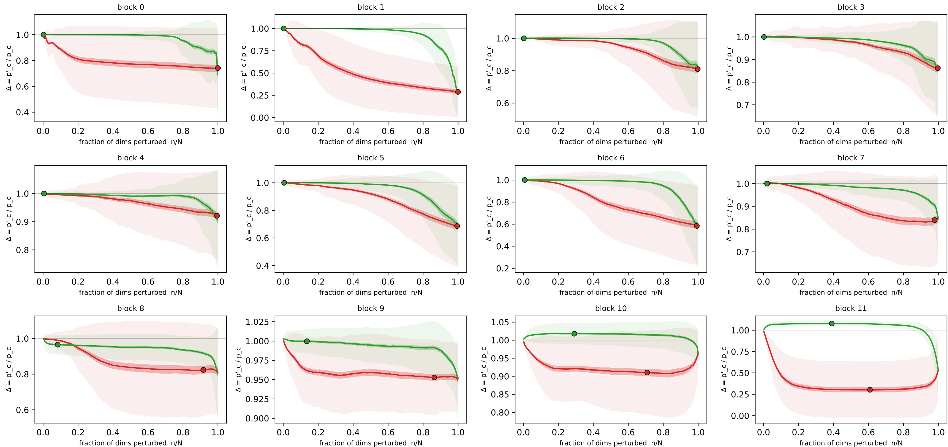
Concept-flipping curves — attnlrp_alpha2beta1 · embed_dim · colored_mnist (n=500 imgs, N=384 detectors) \Delta(n) = target-class prob after perturbing the n most/least relevant detectors, ÷ baseline prob
