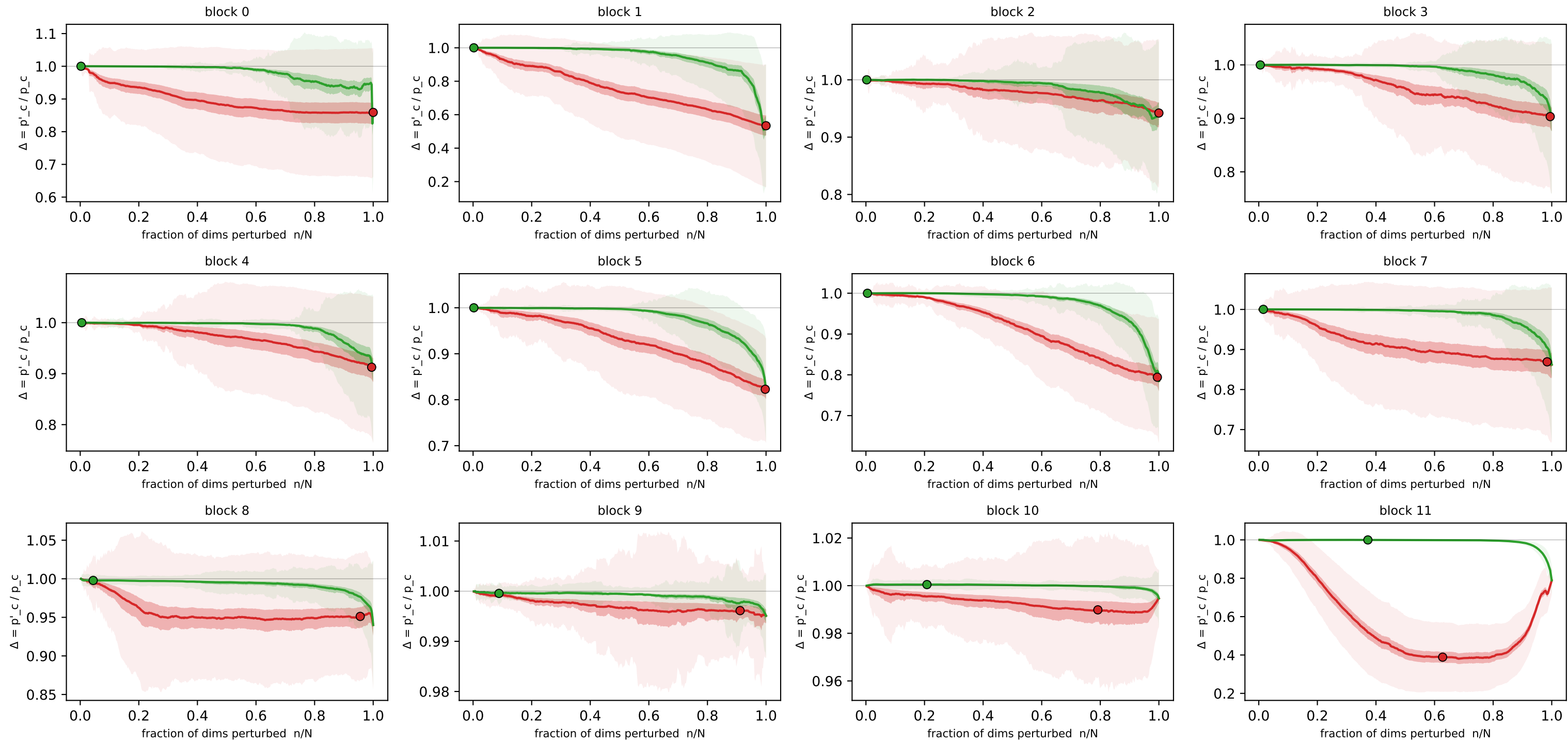
Concept-flipping curves — attnlrp_alpha2beta1 · embed_dim · dsprites (n=150 imgs, N=384 detectors) \Delta(n) = target-class prob after perturbing the n most/least relevant detectors, ÷ baseline prob
