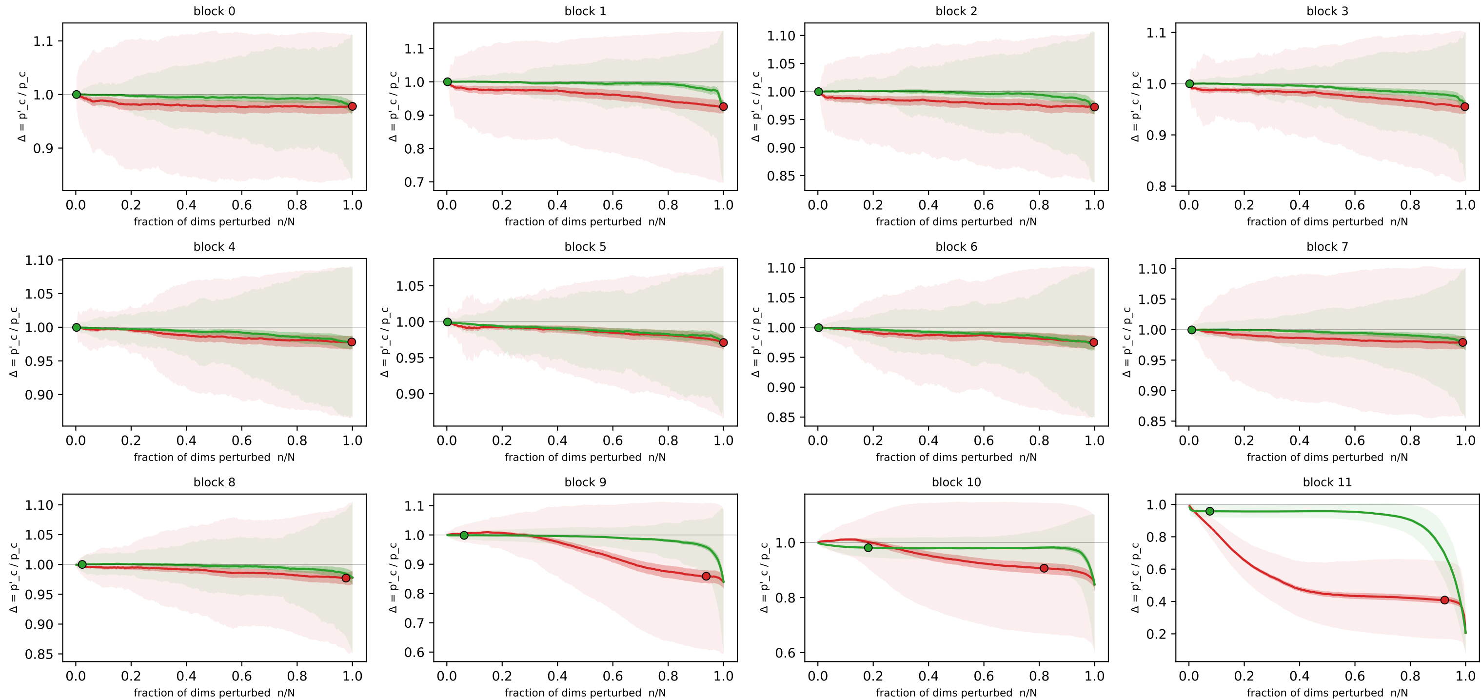
Concept-flipping curves — attnlrp_alpha2beta1 · embed_dim · funny_birds (n=500 imgs, N=384 detectors) \Delta(n) = target-class prob after perturbing the n most/least relevant detectors, ÷ baseline prob
