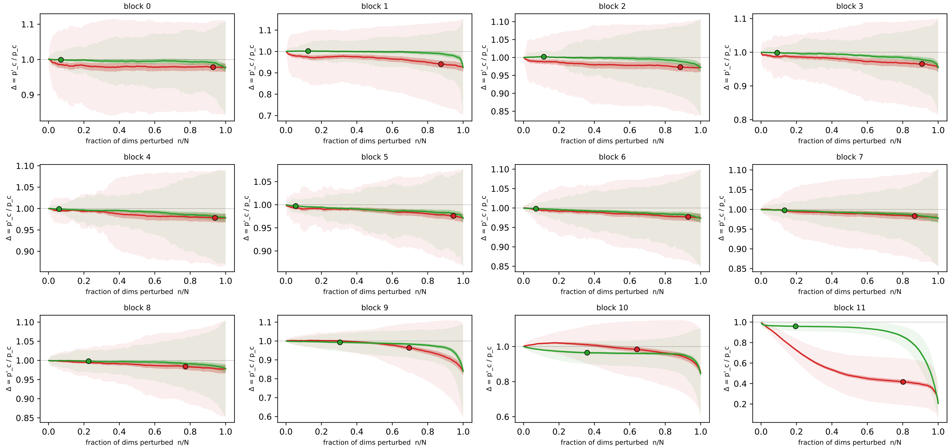
Concept-flipping curves — attnlrp_epsilon · embed_dim · funny_birds (n=500 imgs, N=384 detectors) \Delta(n) = target-class prob after perturbing the n most/least relevant detectors, ÷ baseline prob
