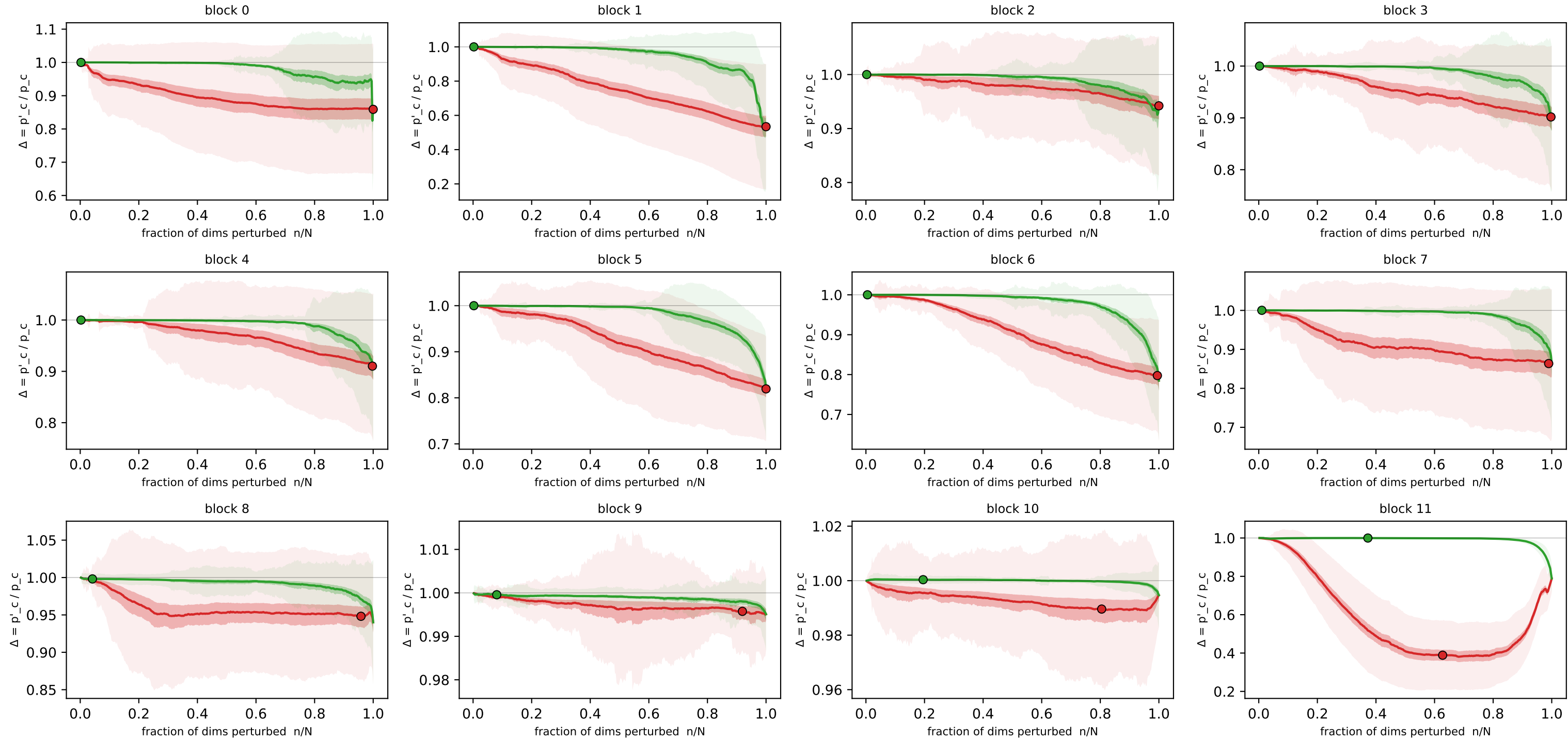
Concept-flipping curves — attnlrp_gamma_palrp · embed_dim · dsprites (n=150 imgs, N=384 detectors) \Delta(n) = target-class prob after perturbing the n most/least relevant detectors, ÷ baseline prob
