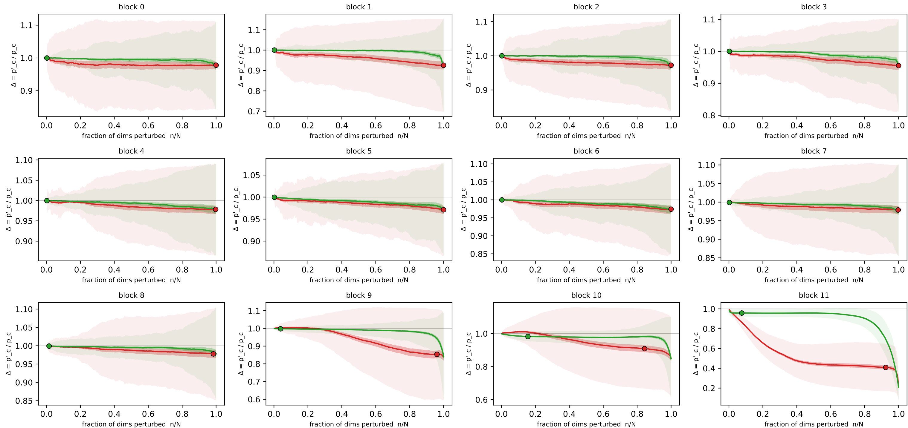
Concept-flipping curves — attnlrp_gamma_palrp · embed_dim · funny_birds (n=500 imgs, N=384 detectors) \Delta(n) = target-class prob after perturbing the n most/least relevant detectors, \div baseline prob
