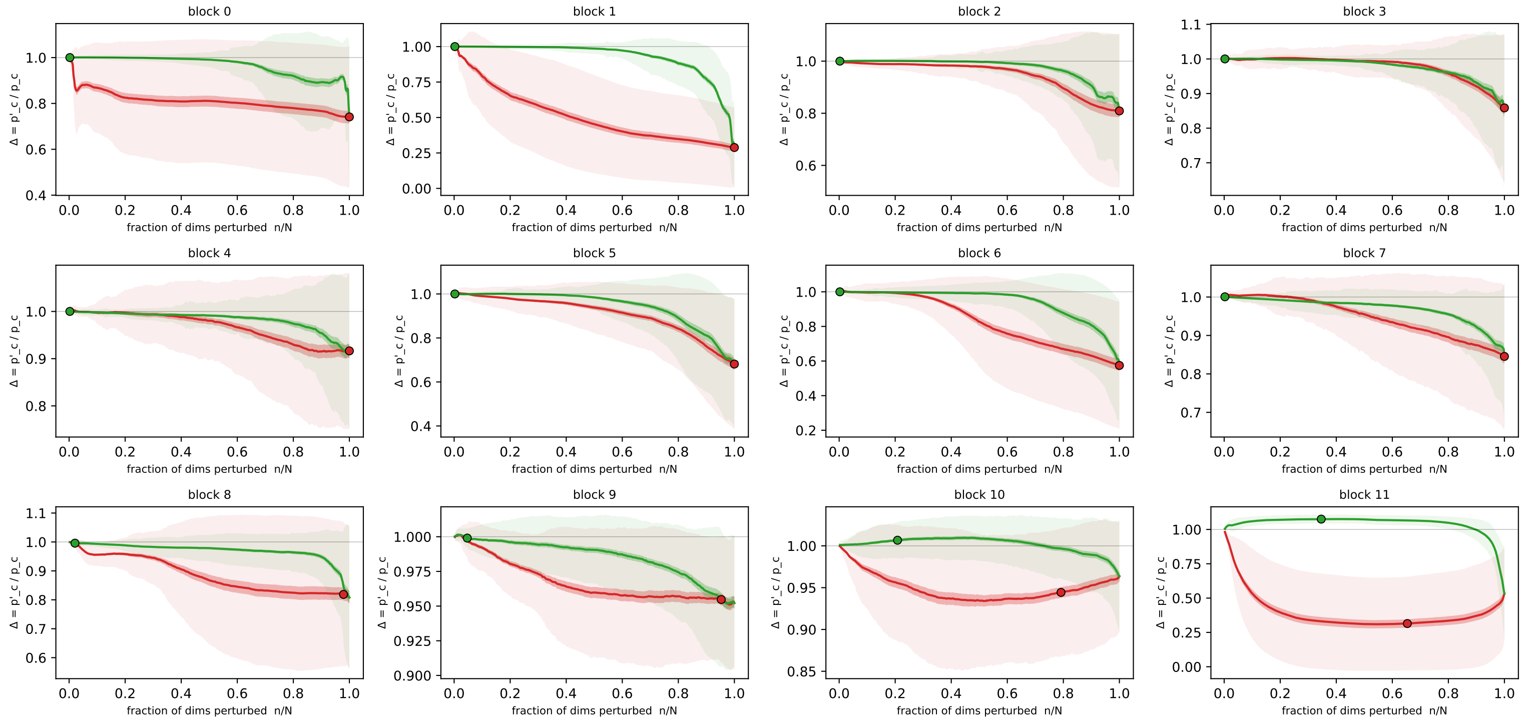
Concept-flipping curves — attnlrp_gamma_residual_none · embed_dim · colored_mnist (n=500 imgs, N=384 detectors) \Delta(n) = target-class prob after perturbing the n most/least relevant detectors, \div baseline prob
