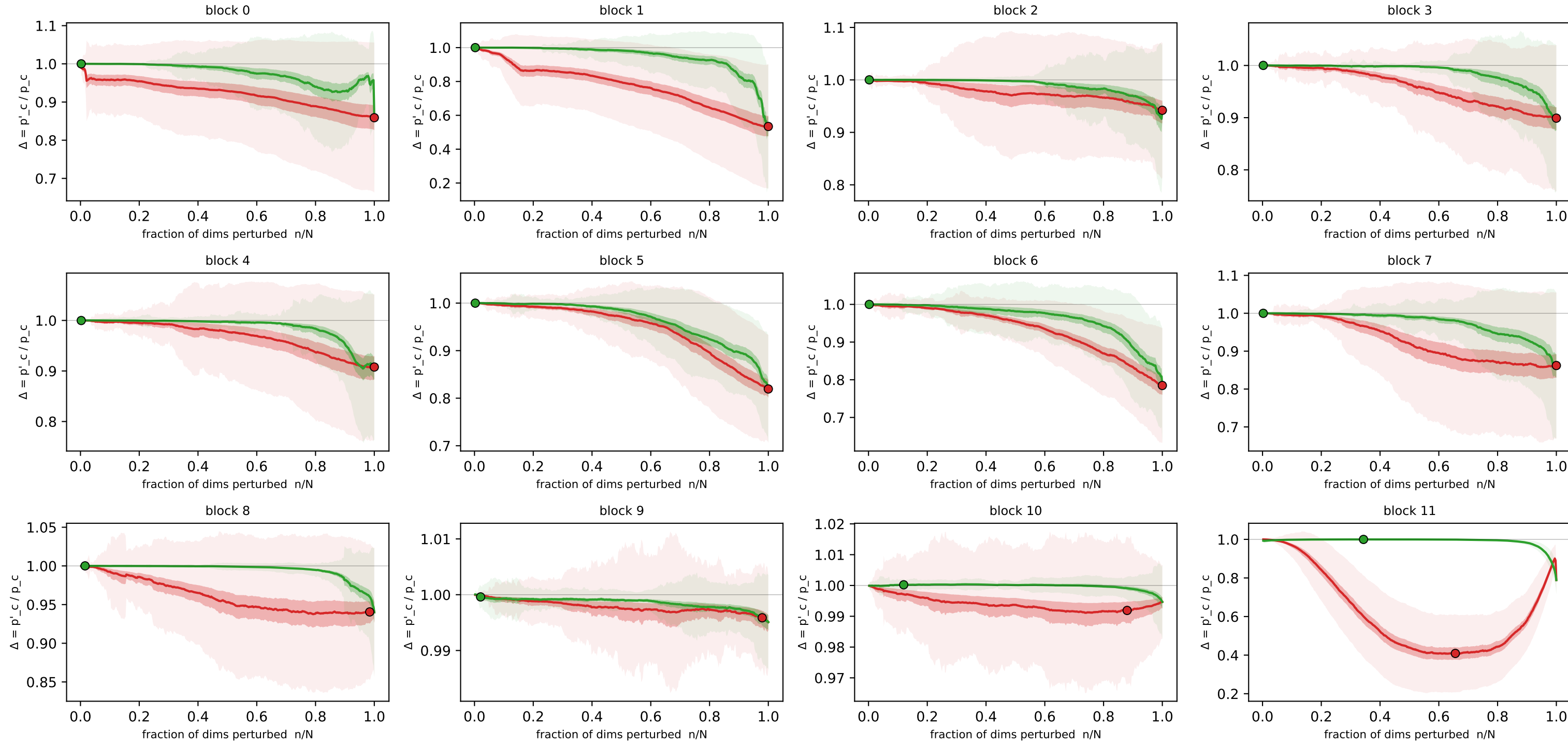
Concept-flipping curves — attnlrp_gamma_residual_none · embed_dim · dsprites (n=150 imgs, N=384 detectors) \Delta(n) = target-class prob after perturbing the n most/least relevant detectors, ÷ baseline prob
