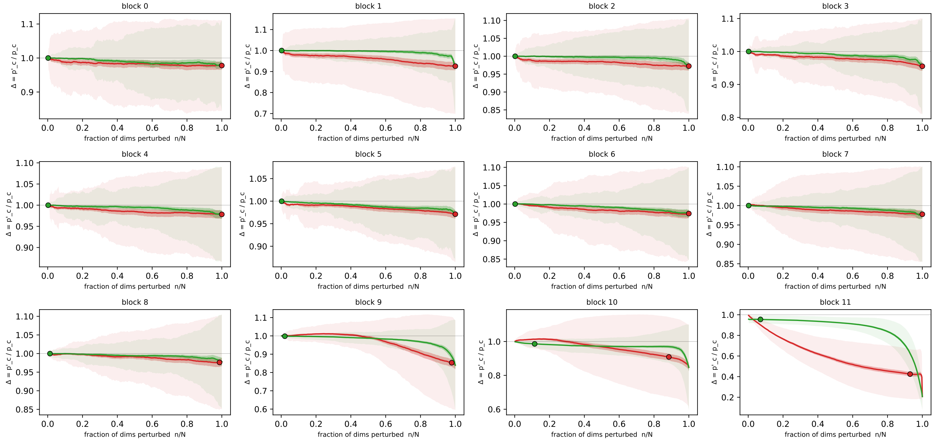
Concept-flipping curves — attnlrp_gamma_residual_none · embed_dim · funny_birds (n=500 imgs, N=384 detectors) \Delta(n) = target-class prob after perturbing the n most/least relevant detectors, ÷ baseline prob
