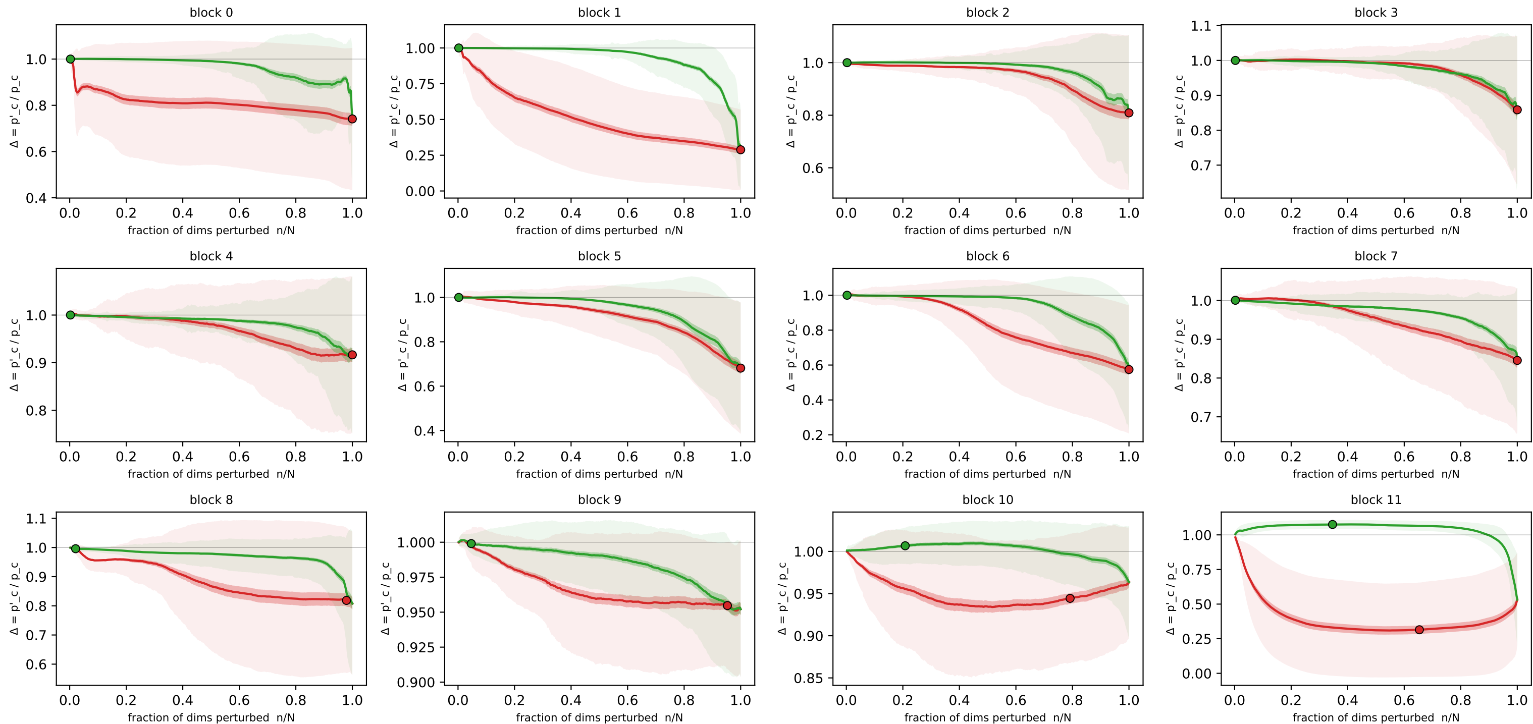
Concept-flipping curves — attnlrp_gamma_residual_symmetric · embed_dim · colored_mnist (n=500 imgs, N=384 detectors) \Delta(n) = target-class prob after perturbing the n most/least relevant detectors, ÷ baseline prob
