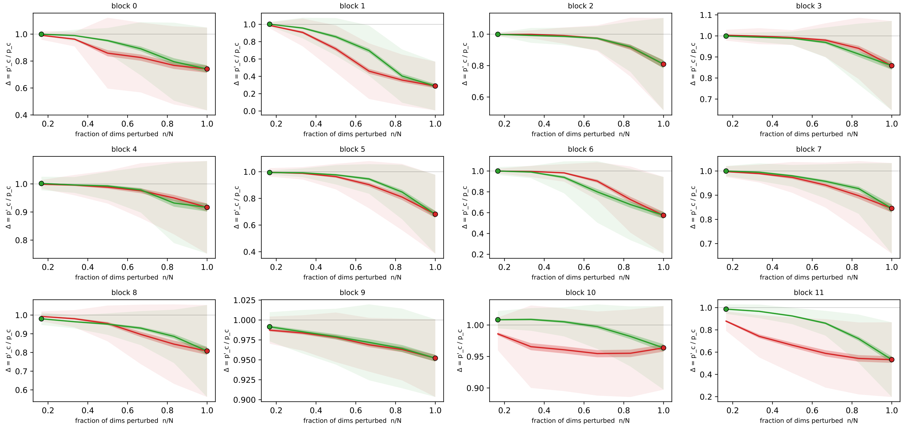
Concept-flipping curves — cp_lrp_baseline · head · colored_mnist (n=500 imgs, N=6 detectors) \Delta(n) = target-class prob after perturbing the n most/least relevant detectors, ÷ baseline prob
