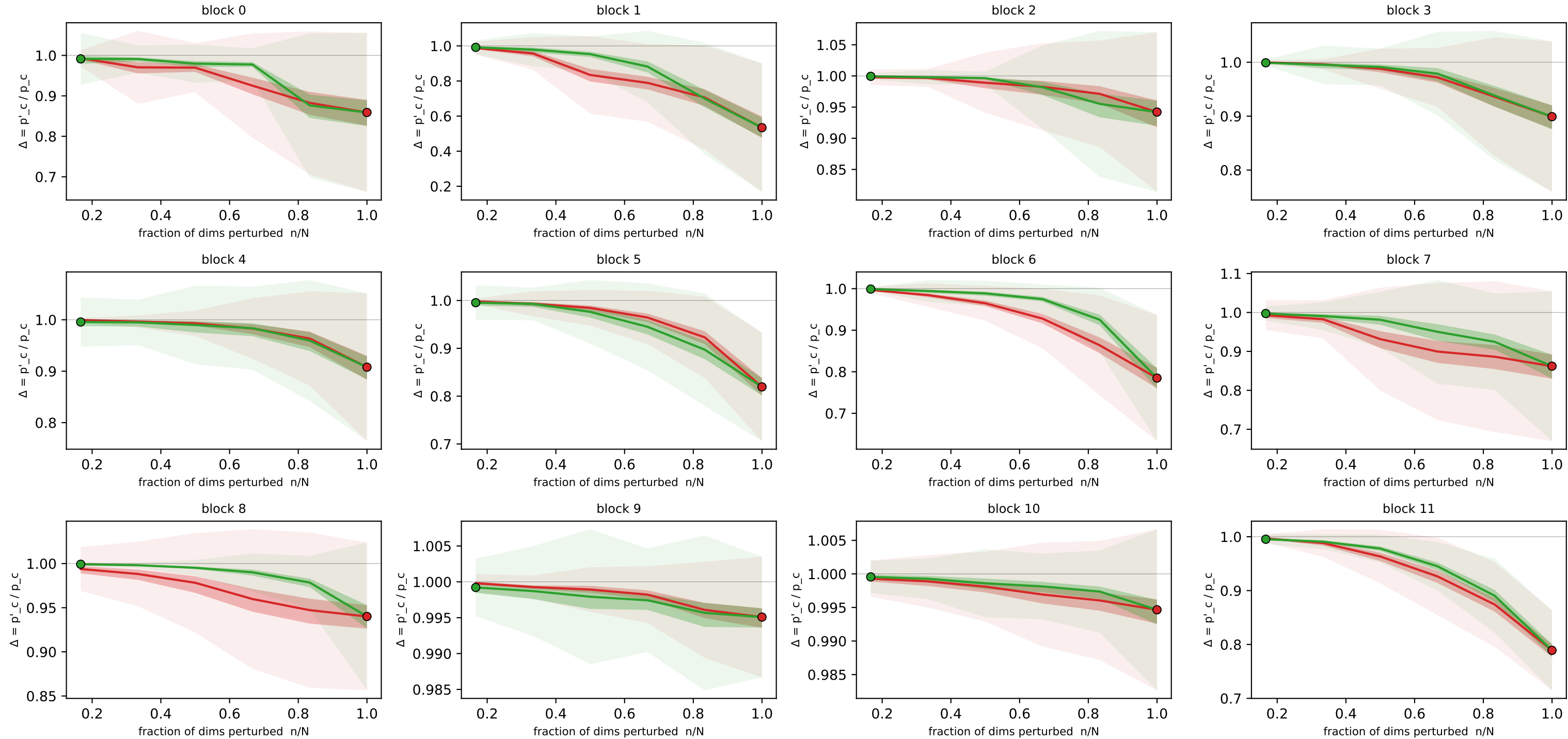
Concept-flipping curves — cp_lrp_baseline · head · dsprites (n=150 imgs, N=6 detectors) \Delta(n) = target-class prob after perturbing the n most/least relevant detectors, ÷ baseline prob
