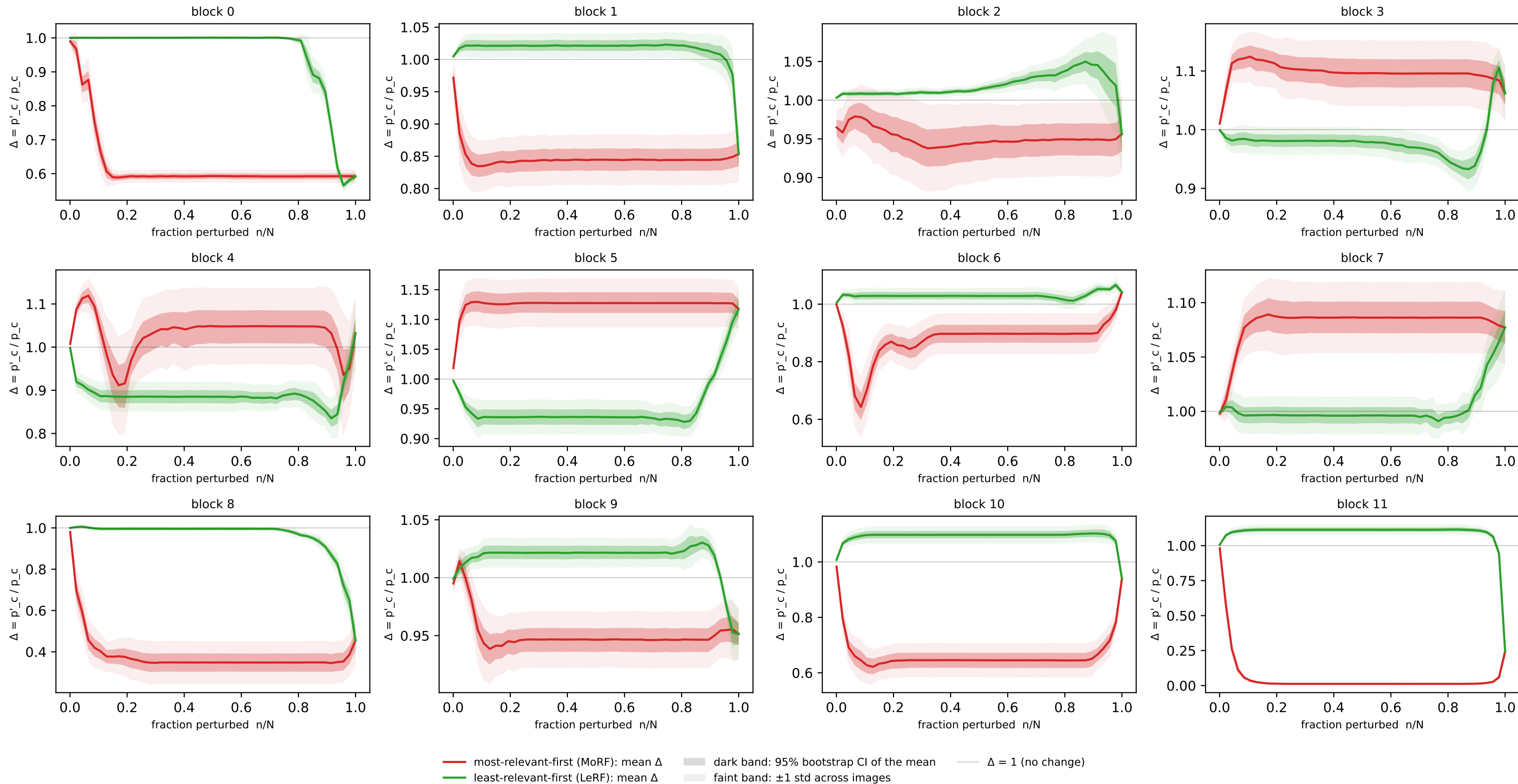
Concept-flipping curves — dsprites · proj_drop · SAE m=1536 (n=20 imgs, N=1536 detectors)
