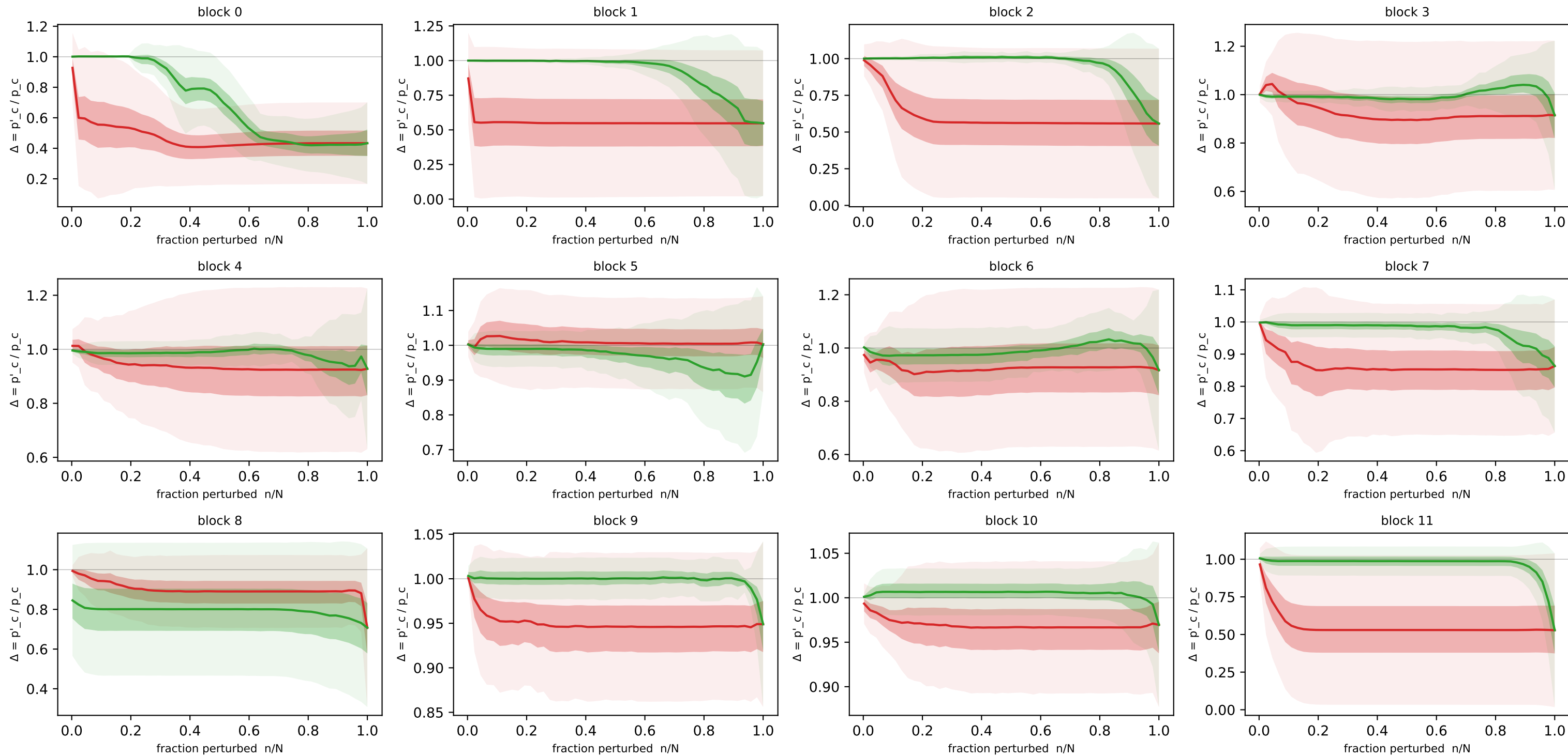
Concept-flipping curves — dsprites · proj_drop · SAE m=384 (n=40 imgs, N=384 detectors)
