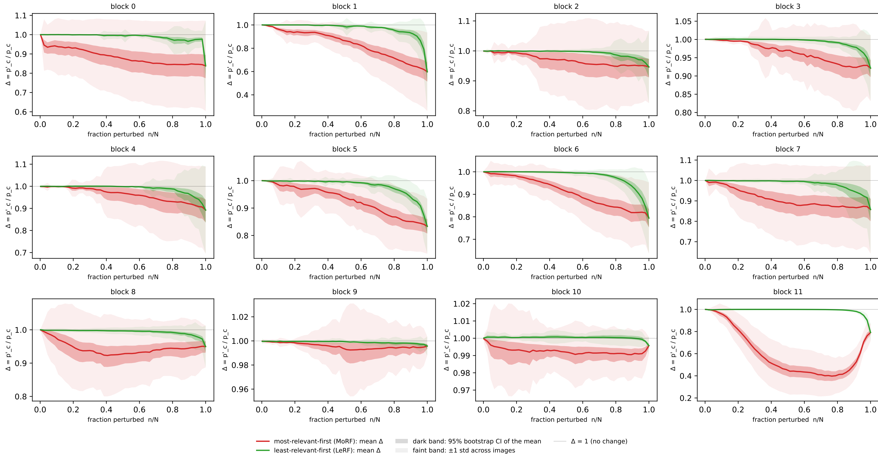
Concept-flipping curves — dsprites · proj_drop · no SAE (axis-aligned, 384) (n=60 imgs, N=384 detectors)
