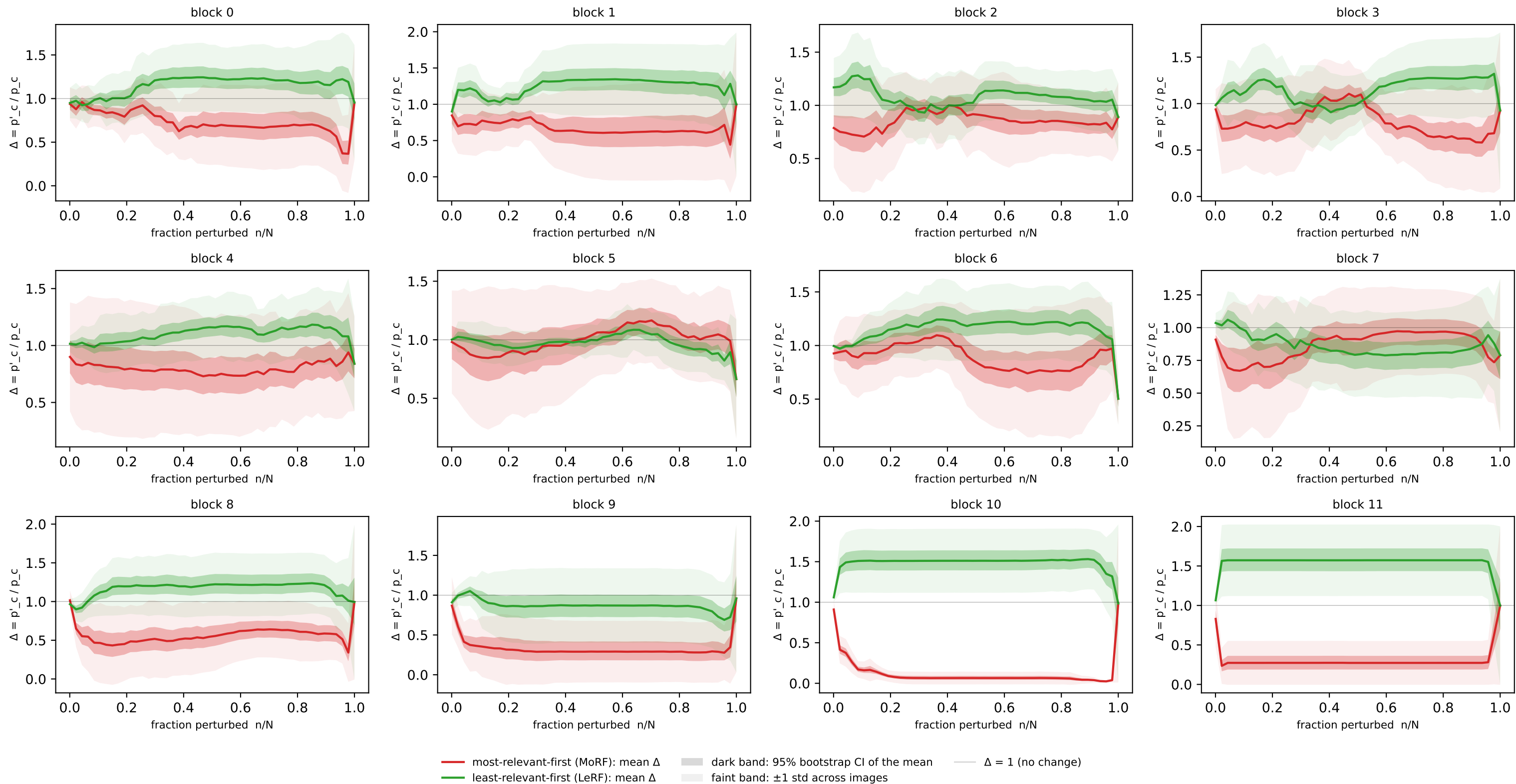
Concept-flipping curves — dsprites · residual · SAE m=1536 (n=40 imgs, N=1536 detectors)
