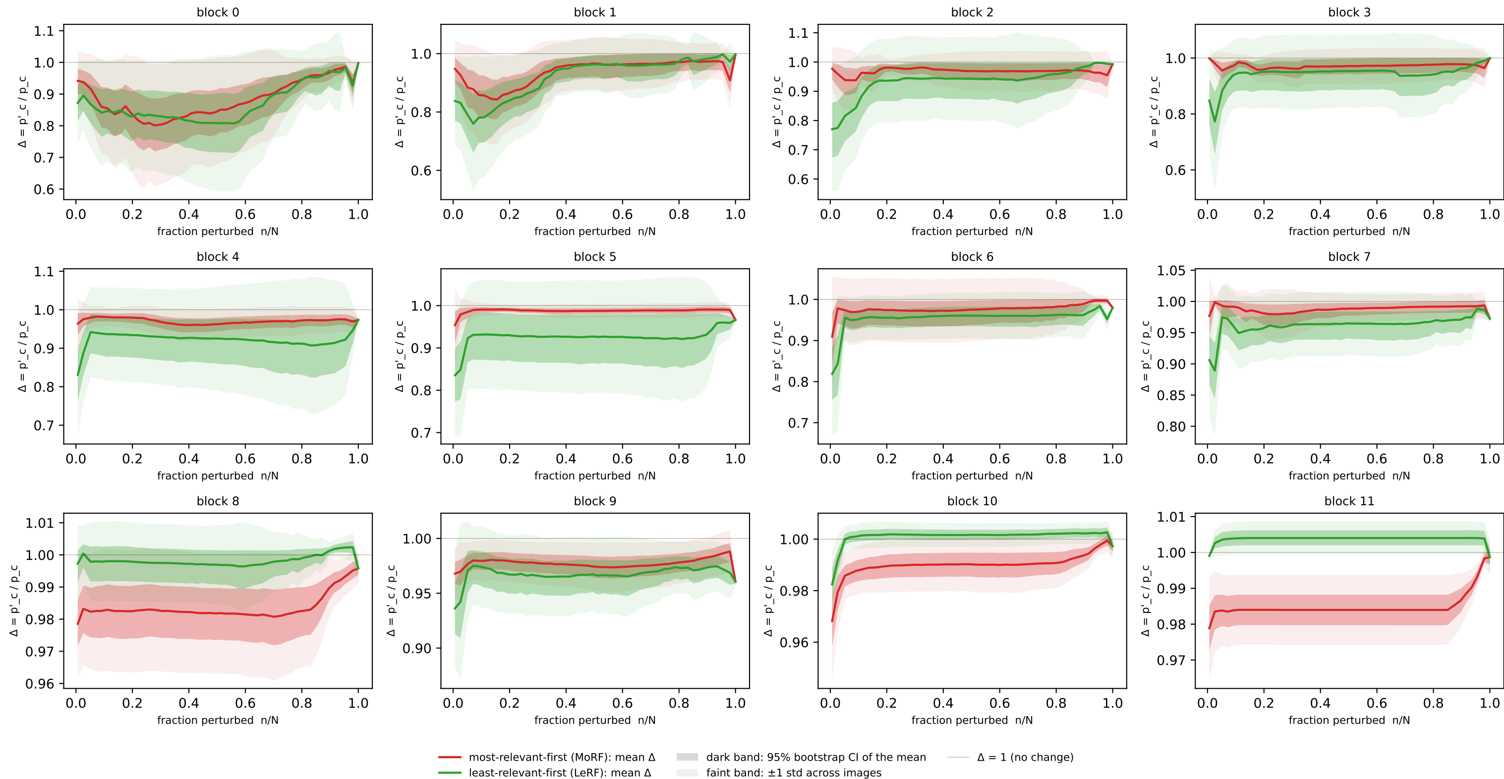
Concept-flipping curves — dsprites · residual · SAE m=154 (n=20 imgs, N=154 detectors)
