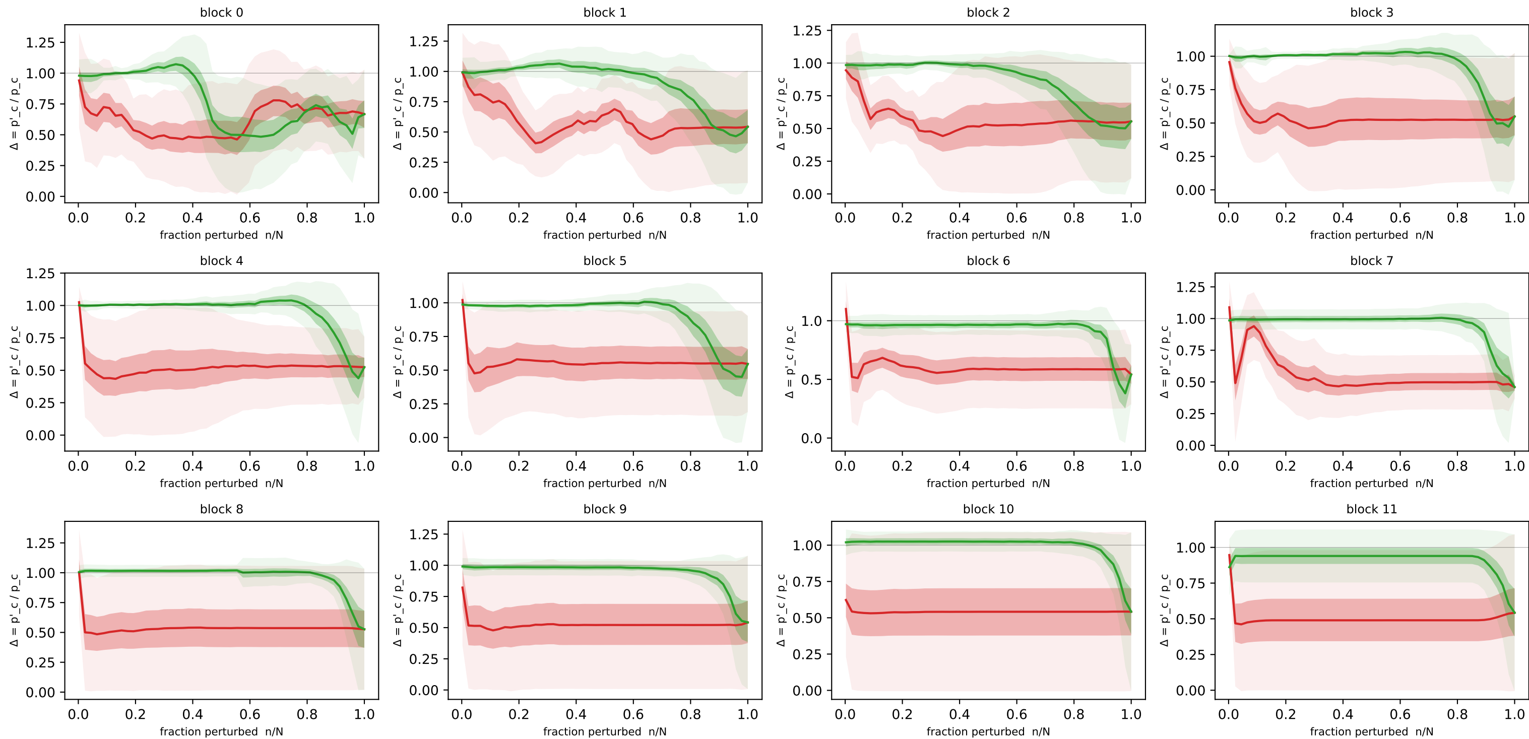
Concept-flipping curves — dsprites · residual · SAE m=384 (n=40 imgs, N=384 detectors)
