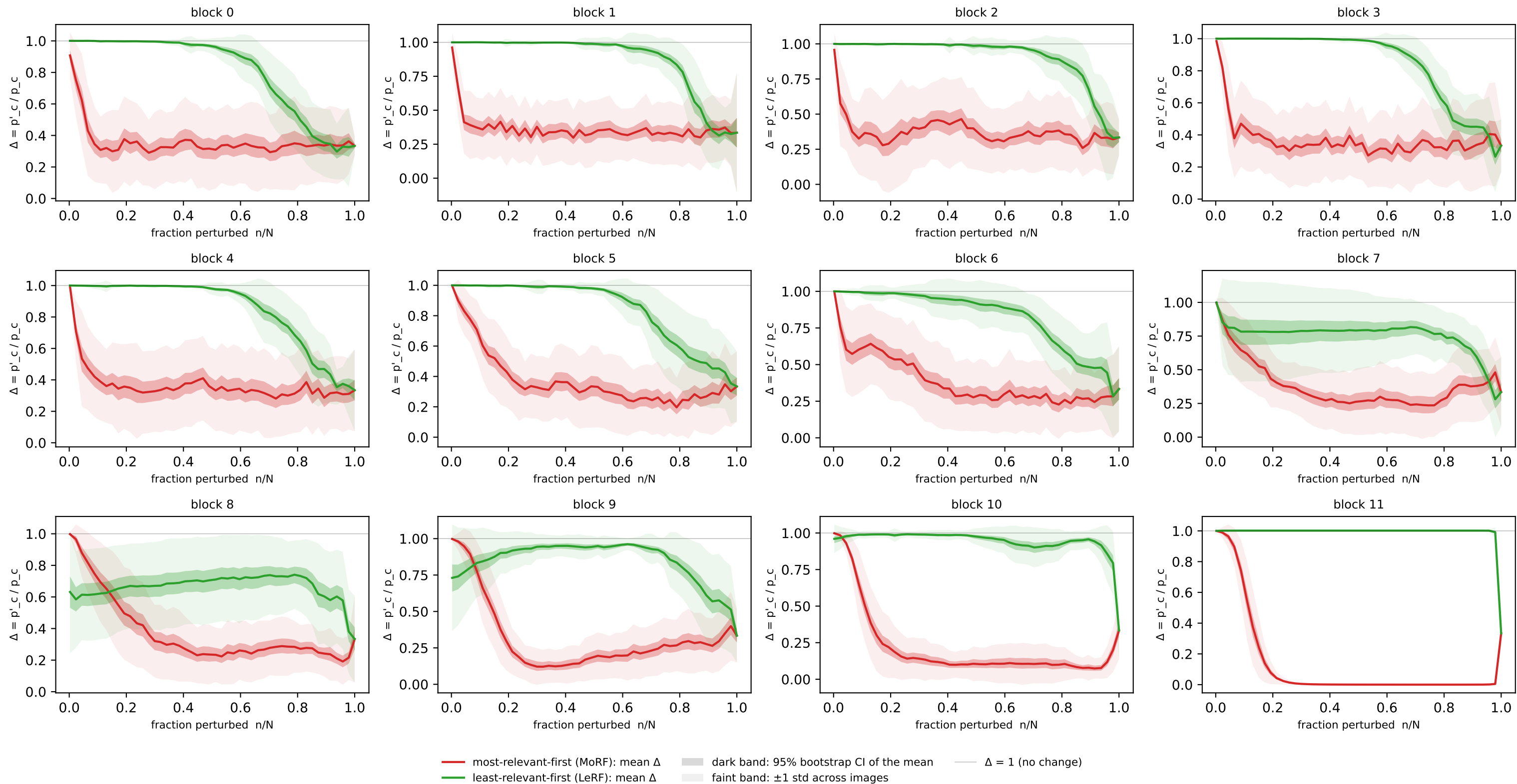
Concept-flipping curves — dsprites · residual · no SAE (axis-aligned, 384) (n=60 imgs, N=384 detectors)
