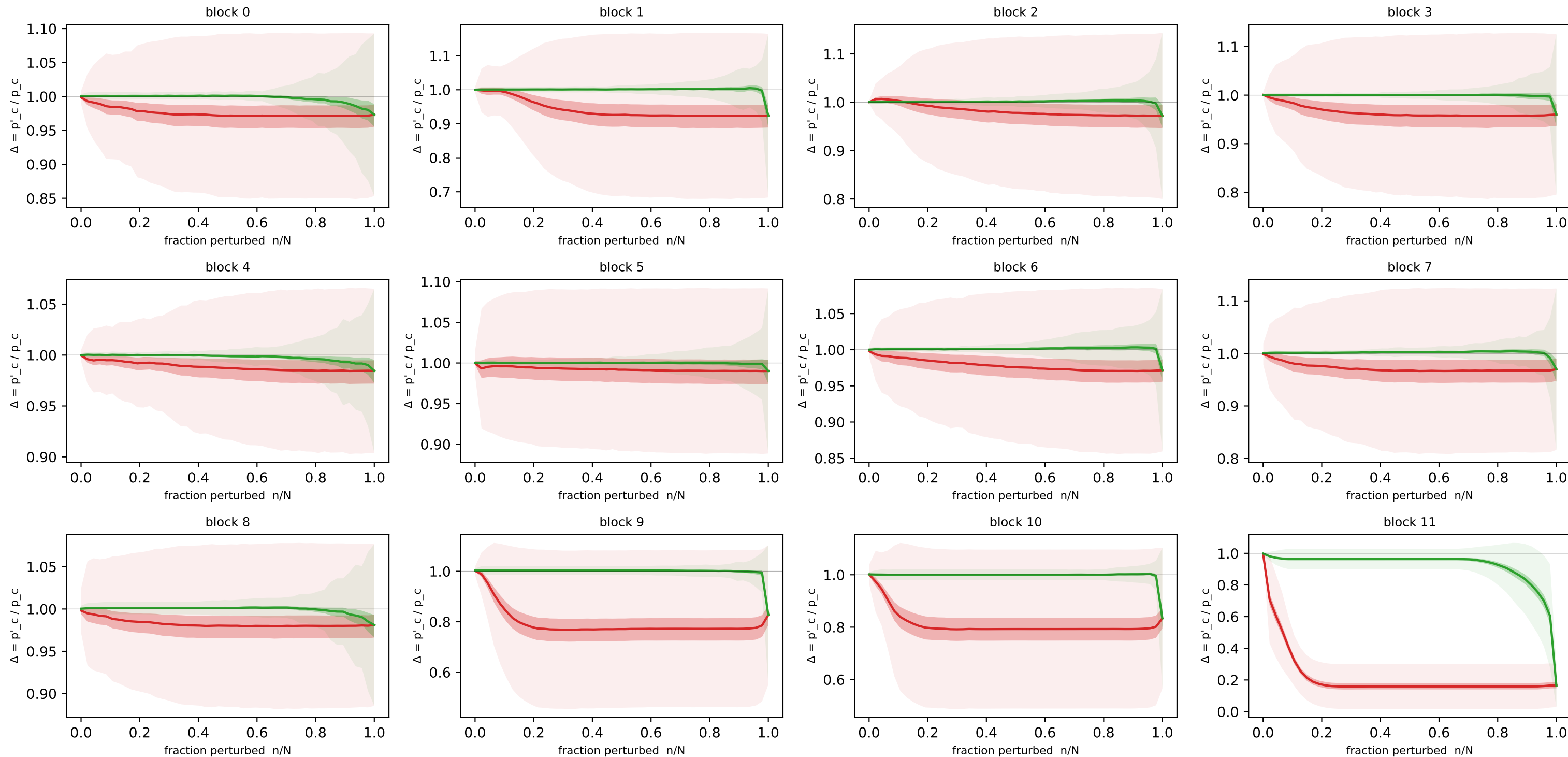
Concept-flipping curves — funny_birds · proj_drop · SAE m=1536 (n=200 imgs, N=1536 detectors)
