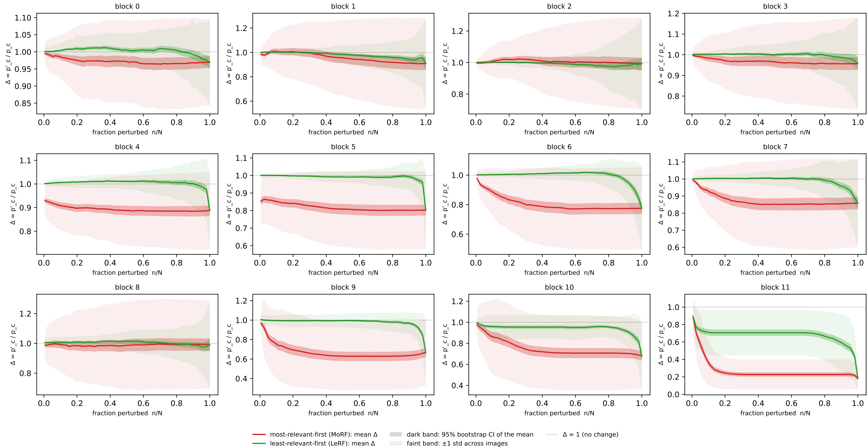
Concept-flipping curves — funny_birds · proj_drop · SAE m=154 (n=200 imgs, N=154 detectors)
