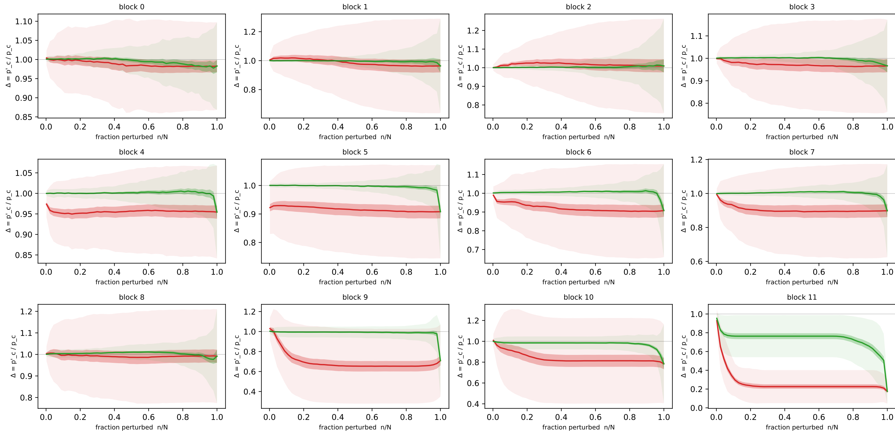
Concept-flipping curves — funny_birds · proj_drop · SAE m=384 (n=200 imgs, N=384 detectors)
