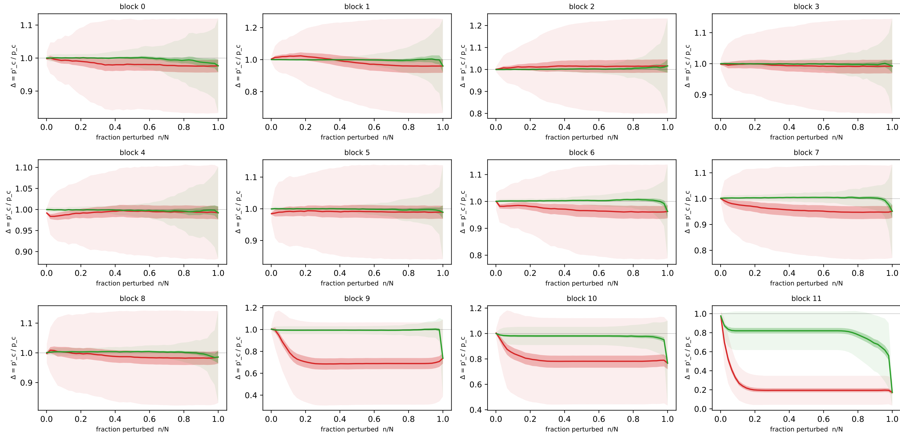
Concept-flipping curves — funny_birds · proj_drop · SAE m=768 (n=200 imgs, N=768 detectors)
